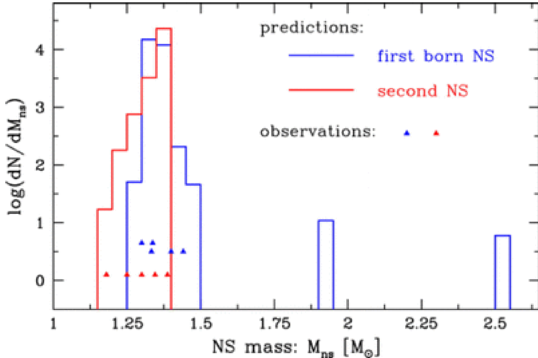
Fig. 3. from The LowestMass Stellar Black Holes: Catastrophic Death of Neutron Stars in GammaRay Bursts Belczynski et al. 2008 ApJL 680 L129 doi:10.1086/589970 https://dx.doi.org/10.1086/589970 © 2008. The American Astronomical Society. All rights reserved. Printed in U.S.A.
