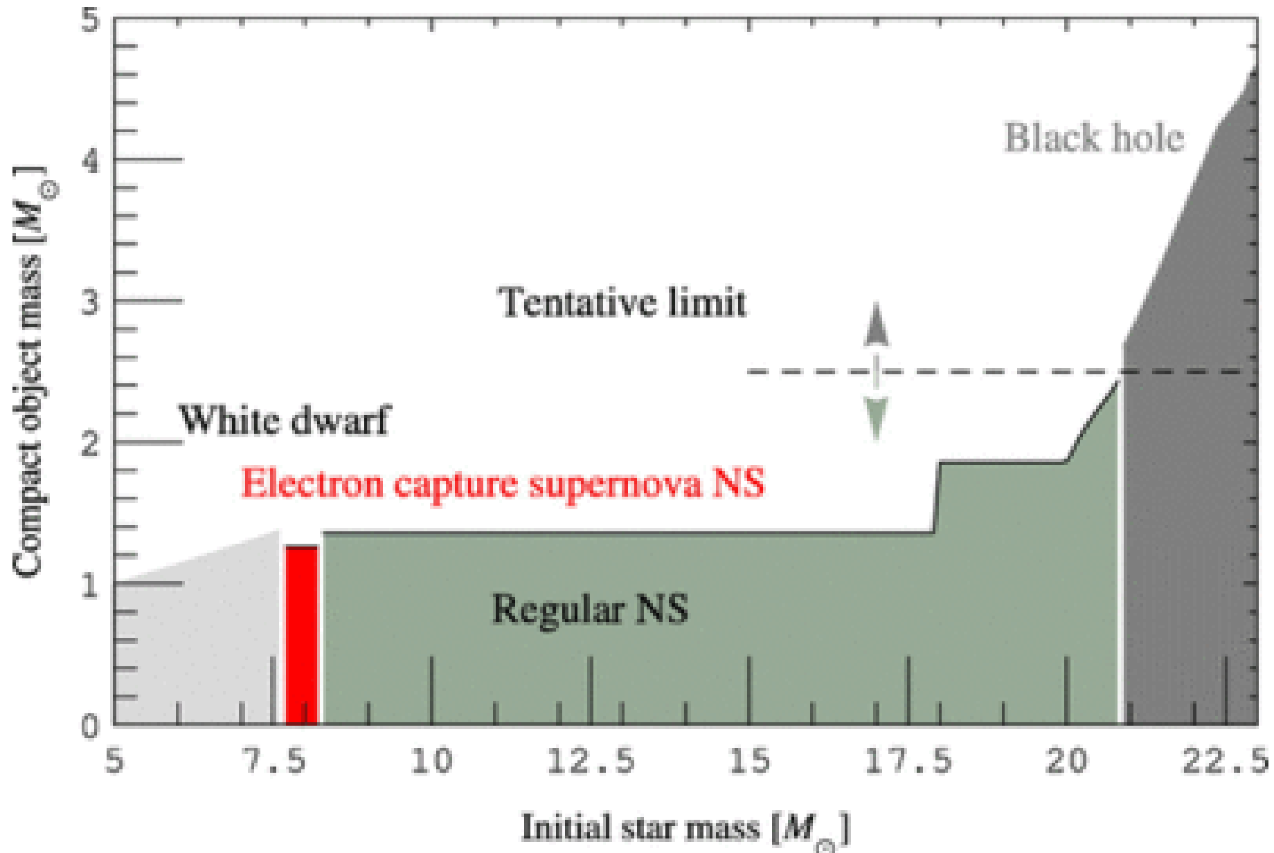
Fig. 2. from The Lowest Mass Stellar Black Holes: Catastrophic Death of Neutron Stars in GammaRay Bursts Belczynski et al. 2008 ApJL 680 L129 doi:10.1086/589970 https://dx.doi.org/10.1086/589970
