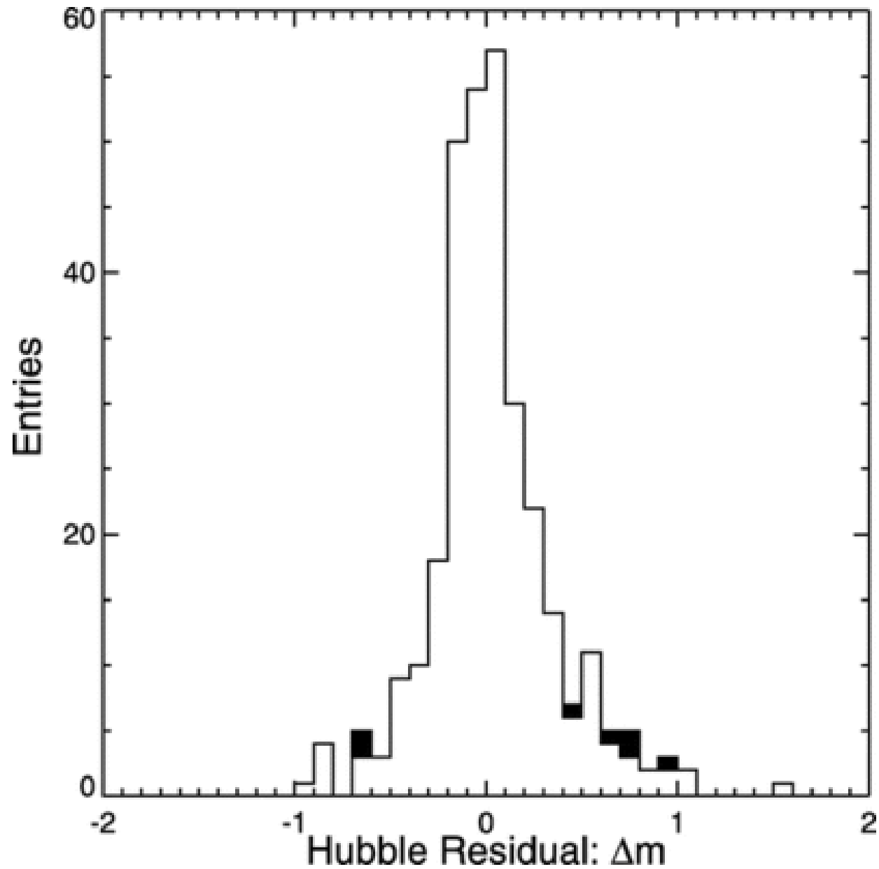
Fig. 6. from Improved Cosmological Constraints from New, Old, and Combined Supernova Data Sets Kowalski et al. 2008 ApJ 686 749 doi:10.1086/589937 https://dx.doi.org/10.1086/589937
