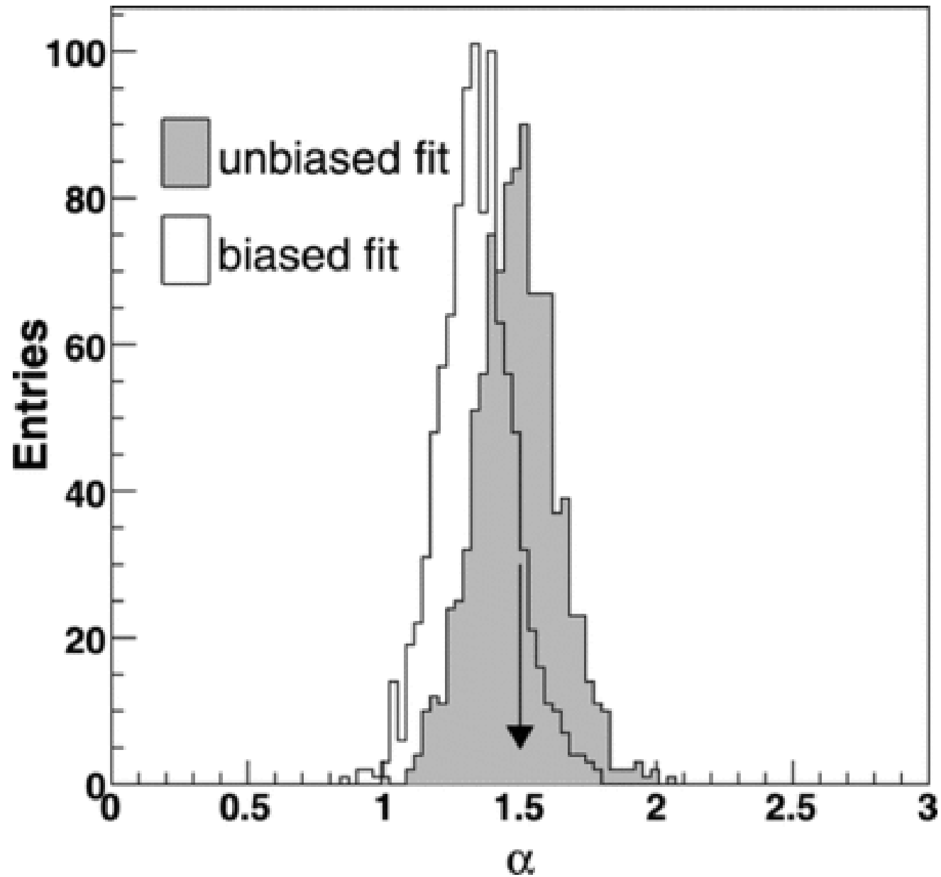
Fig. 5. from Improved Cosmological Constraints from New, Old, and Combined Supernova Data Sets Kowalski et al. 2008 ApJ 686 749 doi:10.1086/589937 https://dx.doi.org/10.1086/589937 © 2008. The American Astronomical Society. All rights reserved. Printed in U.S.A.
