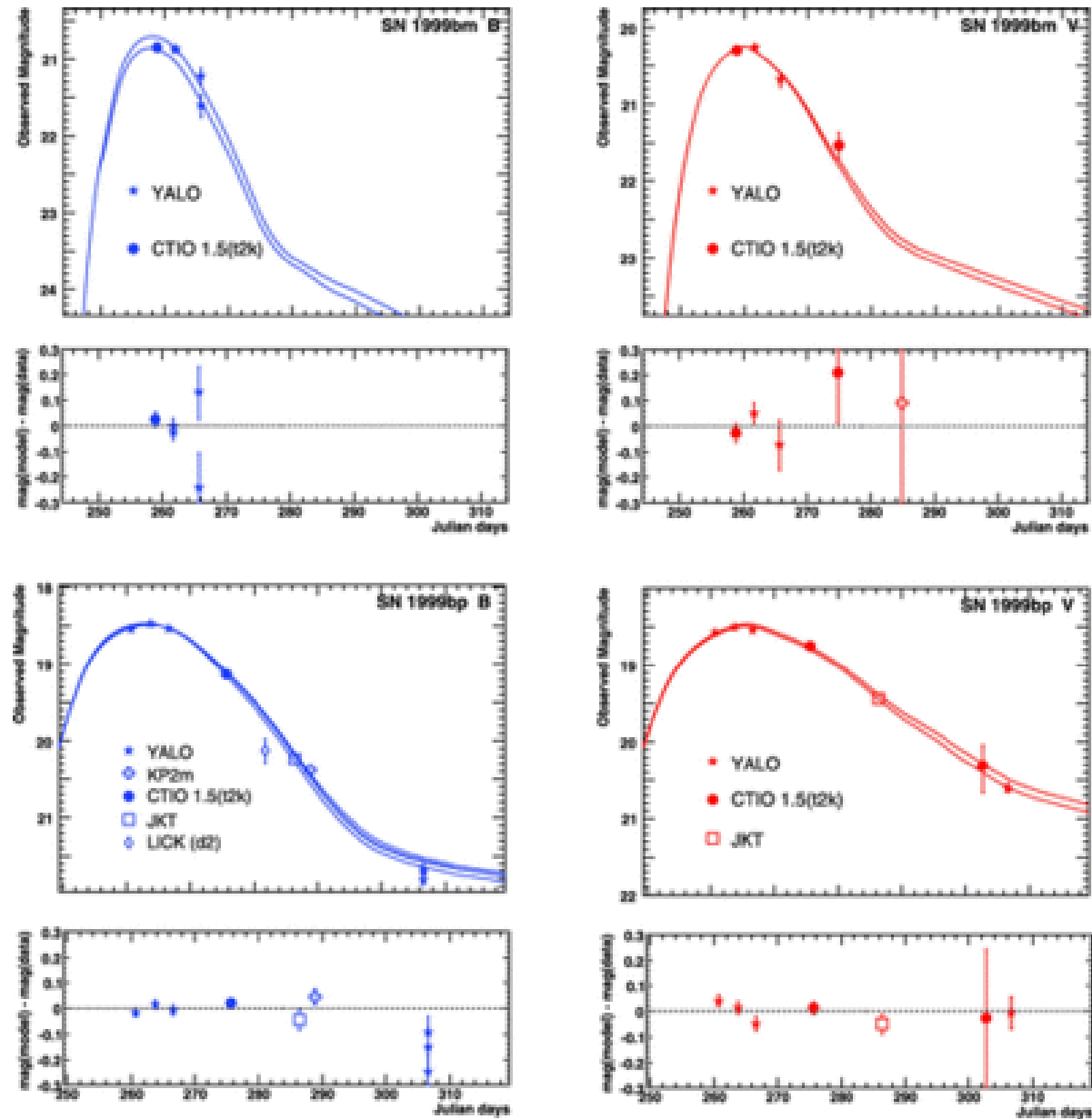
Fig. 3. from Improved Cosmological Constraints from New, Old, and Combined Supernova Data Sets Kowalski et al. 2008 ApJ 686 749 doi:10.1086/589937 https://dx.doi.org/10.1086/589937
