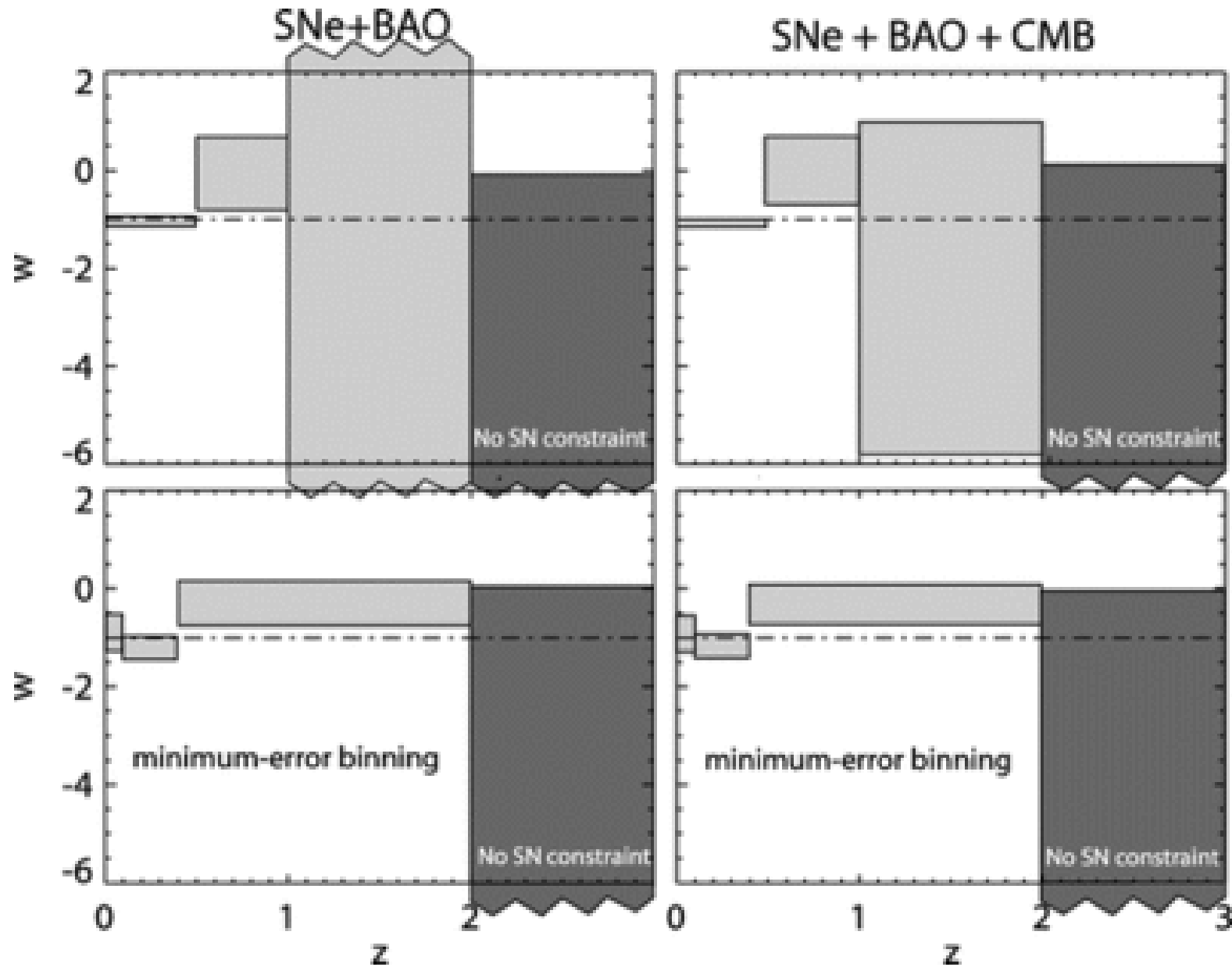
Fig. 17. from Improved Cosmological Constraints from New, Old, and Combined Supernova Data Sets Kowalski et al. 2008 ApJ 686 749 doi:10.1086/589937 https://dx.doi.org/10.1086/589937 © 2008. The American Astronomical Society. All rights reserved. Printed in U.S.A.
