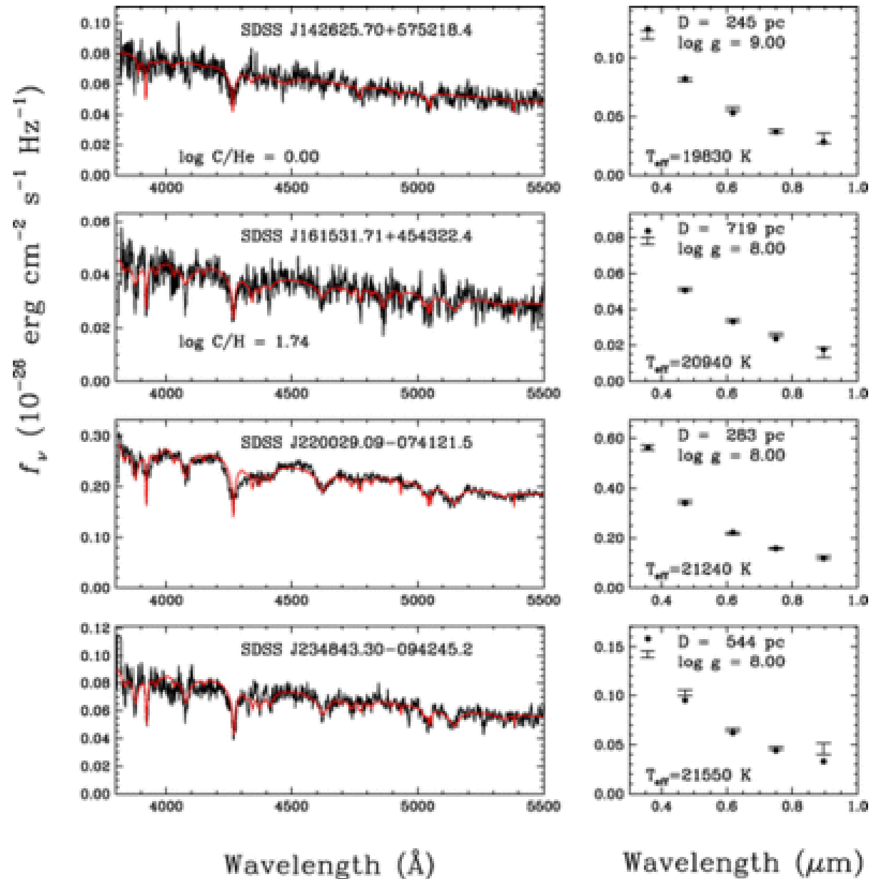
Fig. 3. from Hot DQ White Dwarfs: Something Different Dufour et al. 2008 ApJ 683 978 doi:10.1086/589855 https://dx.doi.org/10.1086/589855
