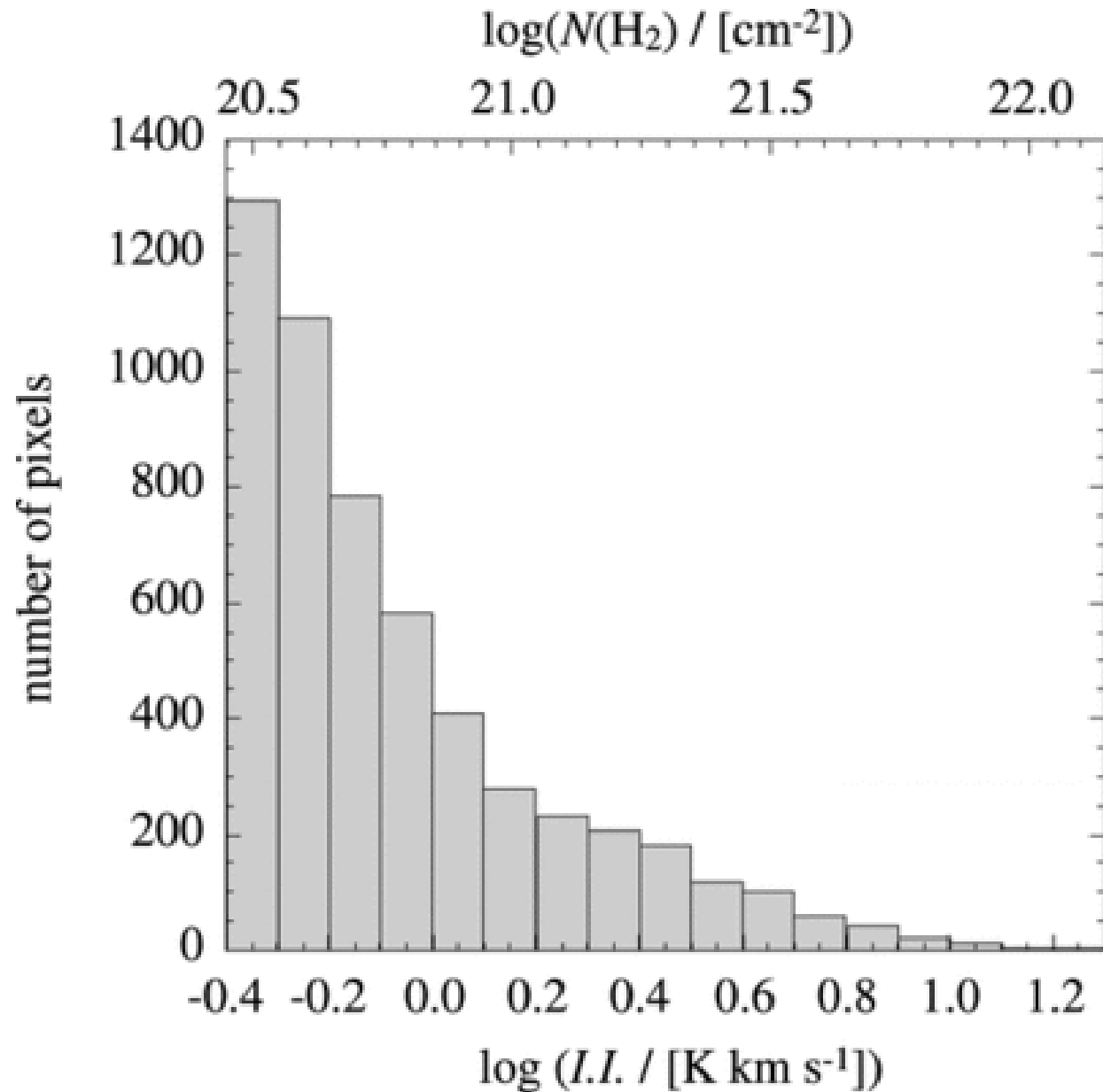
Fig. 3. from The Second Survey of the Molecular Clouds in the Large Magellanic Cloud by NANTEN. I. Catalog of Molecular Clouds Fukui et al. 2008 ApJS 178 56 doi:10.1086/589833 https://dx.doi.org/10.1086/589833
