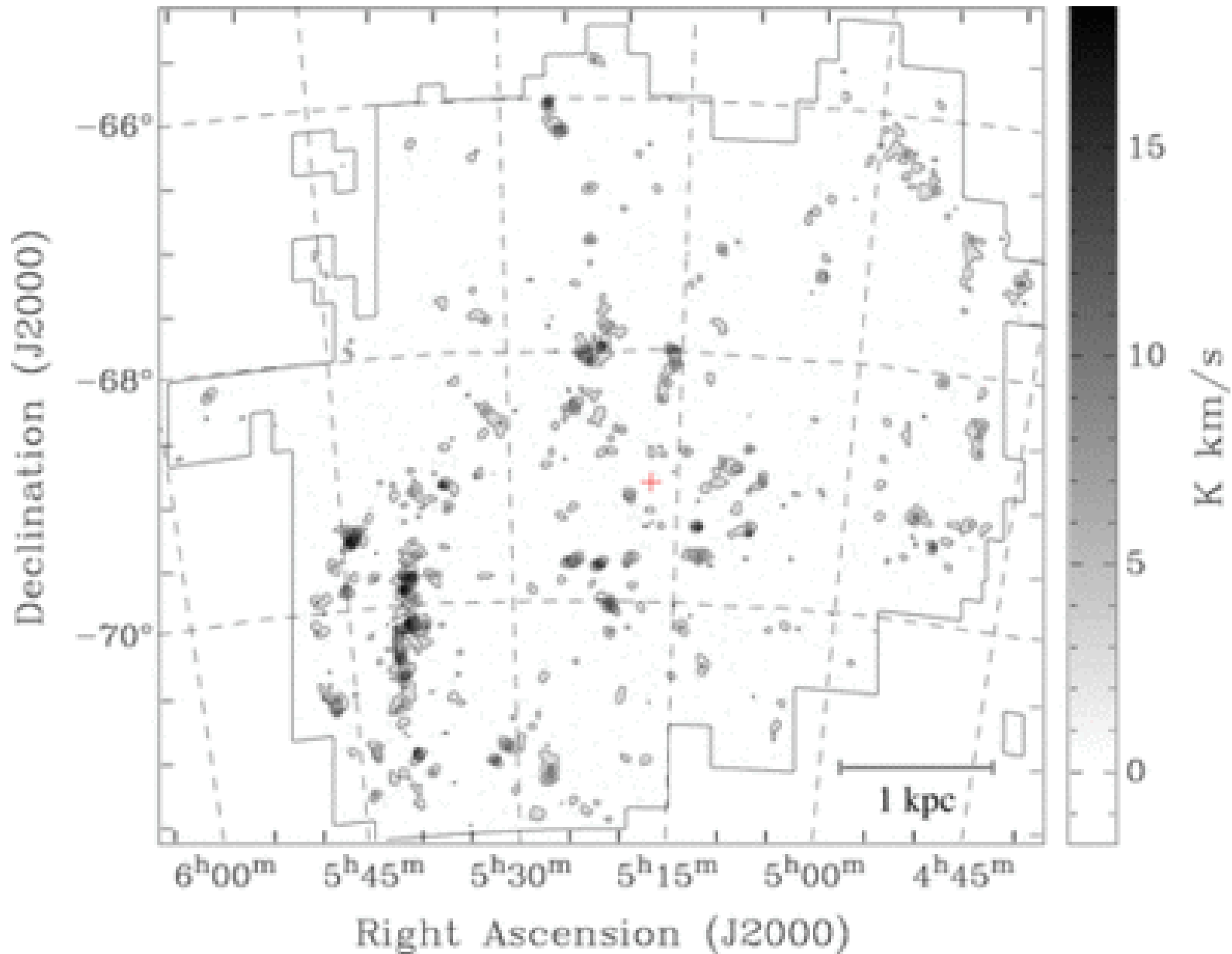
Fig. 2. from The Second Survey of the Molecular Clouds in the Large Magellanic Cloud by NANTEN. I. Catalog of Molecular Clouds Fukui et al. 2008 ApJS 178 56 doi:10.1086/589833 https://dx.doi.org/10.1086/589833 © 2008. The American Astronomical Society. All rights reserved. Printed in U.S.A.
