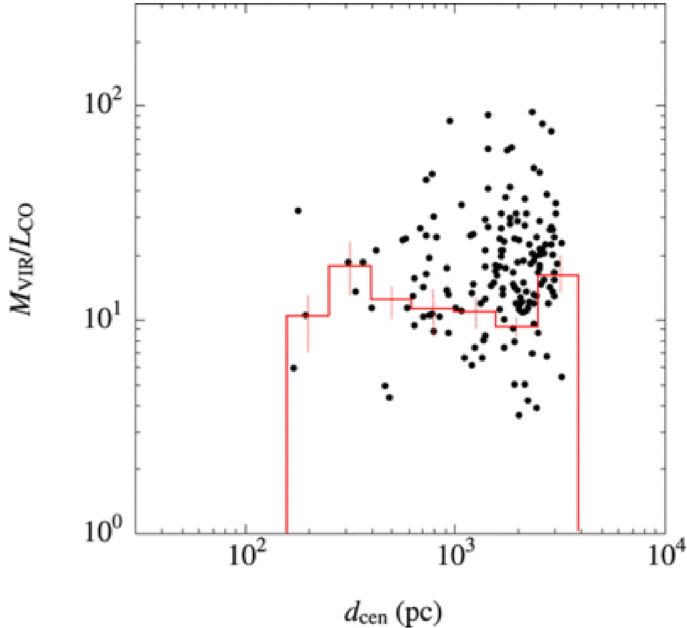
Fig. 18. from The Second Survey of the Molecular Clouds in the Large Magellanic Cloud by NANTEN. I. Catalog of Molecular Clouds Fukui et al. 2008 ApJS 178 56 doi:10.1086/589833 https://dx.doi.org/10.1086/589833 © 2008. The American Astronomical Society. All rights reserved. Printed in U.S.A.
