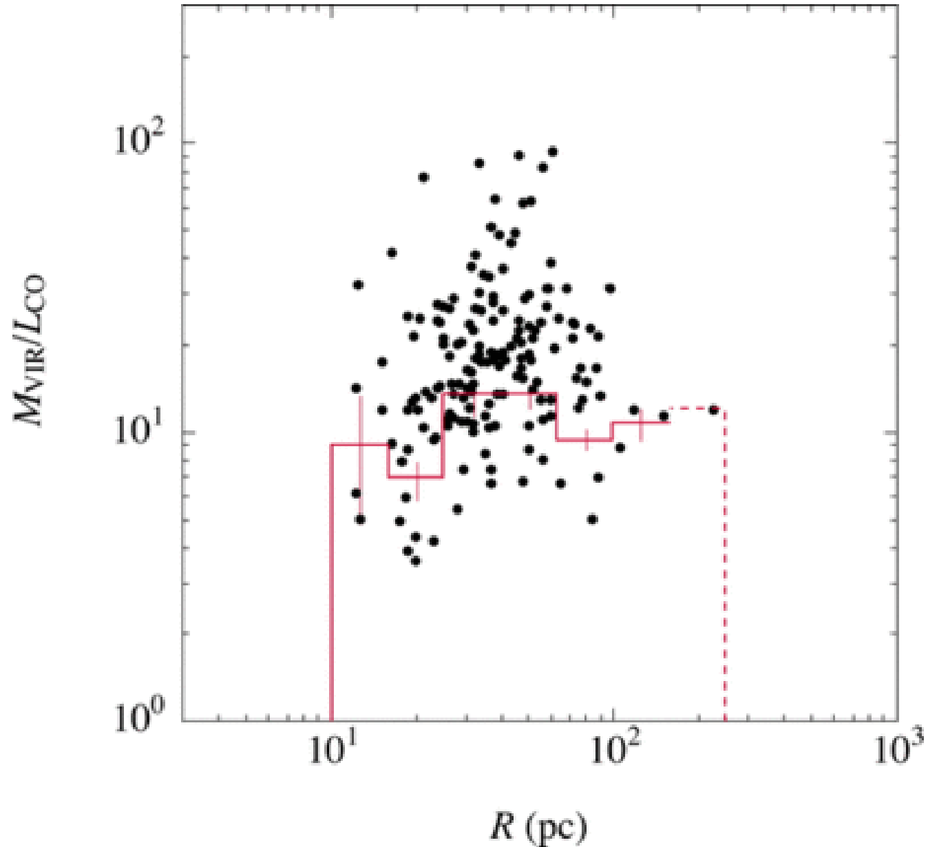
Fig. 17. from The Second Survey of the Molecular Clouds in the Large Magellanic Cloud by NANTEN. I. Catalog of Molecular Clouds Fukui et al. 2008 ApJS 178 56 doi:10.1086/589833 https://dx.doi.org/10.1086/589833 © 2008. The American Astronomical Society. All rights reserved. Printed in U.S.A.
