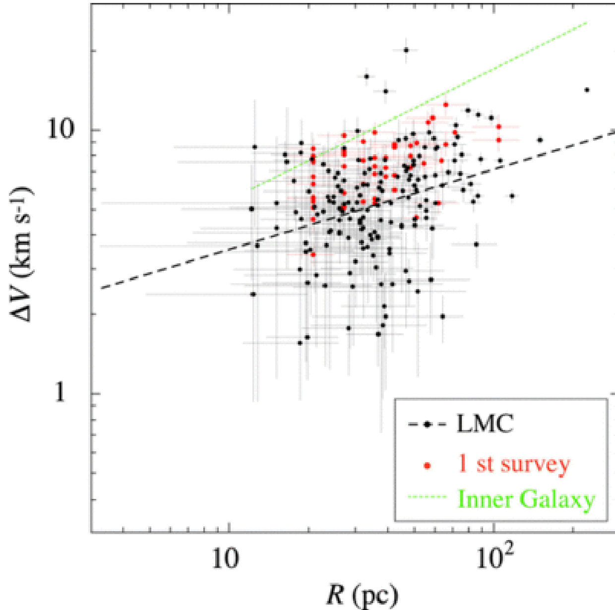
Fig. 14. from The Second Survey of the Molecular Clouds in the Large Magellanic Cloud by NANTEN. I. Catalog of Molecular Clouds Fukui et al. 2008 ApJS 178 56 doi:10.1086/589833 https://dx.doi.org/10.1086/589833 © 2008. The American Astronomical Society. All rights reserved. Printed in U.S.A.
