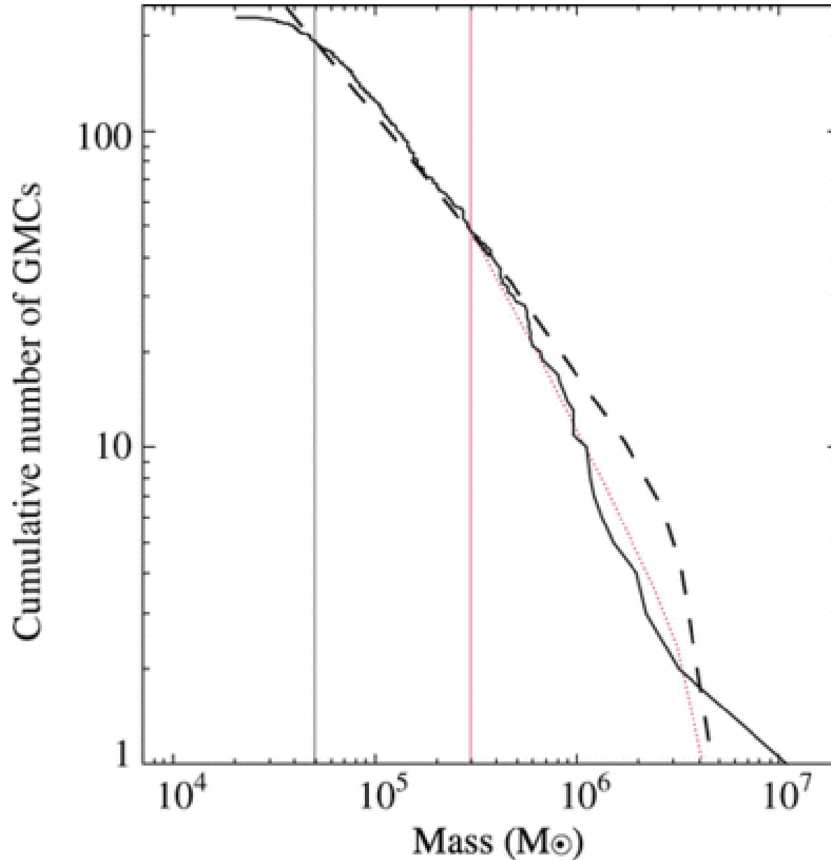
Fig. 13. from The Second Survey of the Molecular Clouds in the Large Magellanic Cloud by NANTEN. I. Catalog of Molecular Clouds Fukui et al. 2008 ApJS 178 56 doi:10.1086/589833 https://dx.doi.org/10.1086/589833 © 2008. The American Astronomical Society. All rights reserved. Printed in U.S.A.
