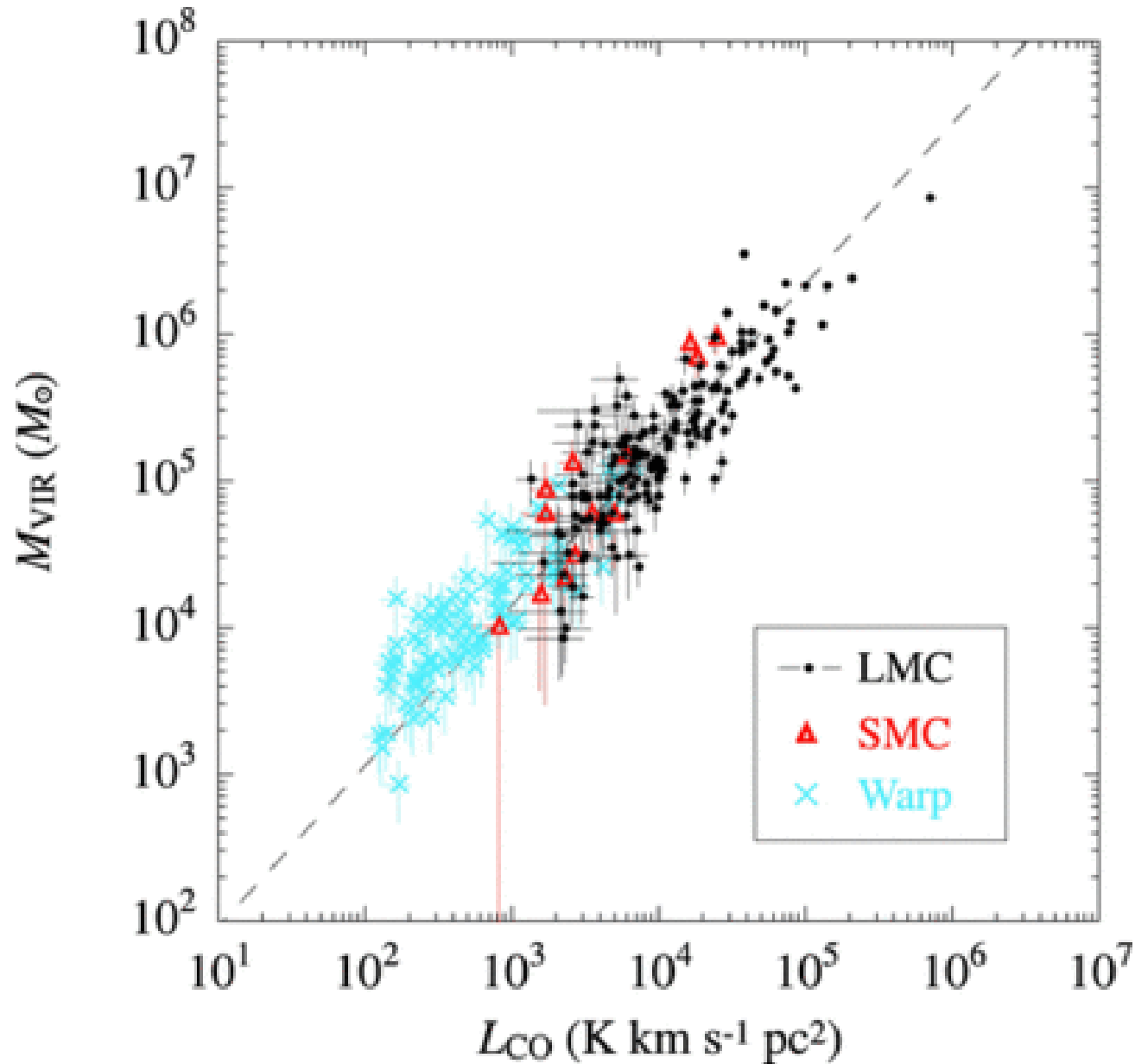
Fig. 12. from The Second Survey of the Molecular Clouds in the Large Magellanic Cloud by NANTEN. I. Catalog of Molecular Clouds Fukui et al. 2008 ApJS 178 56 doi:10.1086/589833 https://dx.doi.org/10.1086/589833
