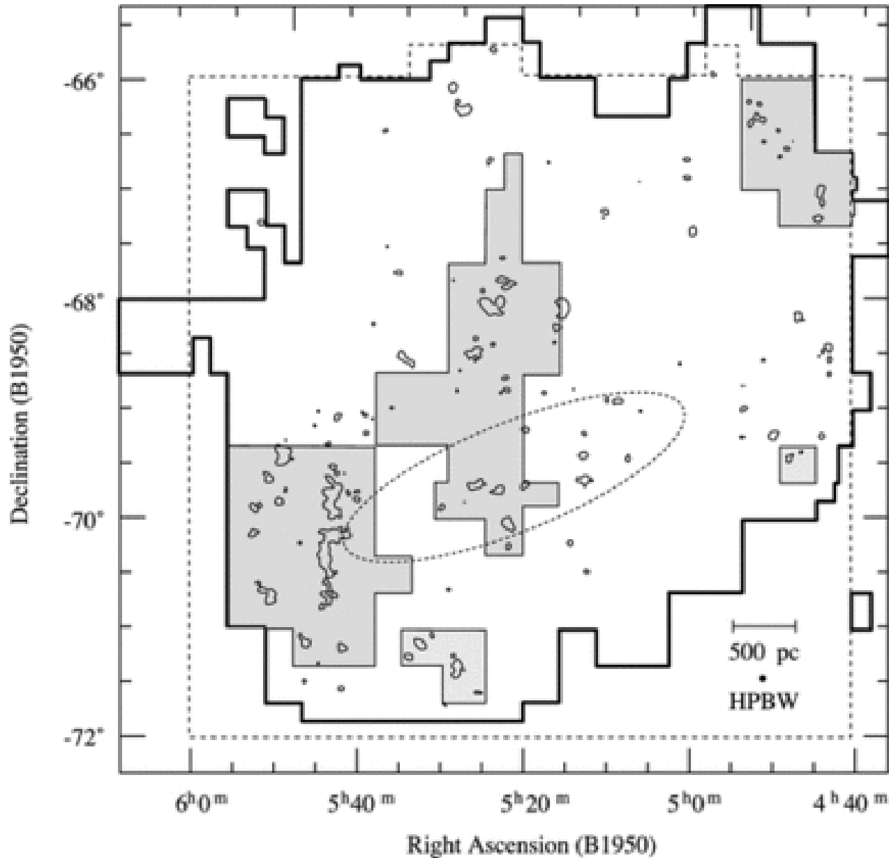
Fig. 1. from The Second Survey of the Molecular Clouds in the Large Magellanic Cloud by NANTEN. I. Catalog of Molecular Clouds Fukui et al. 2008 ApJS 178 56 doi:10.1086/589833 https://dx.doi.org/10.1086/589833 © 2008. The American Astronomical Society. All rights reserved. Printed in U.S.A.
