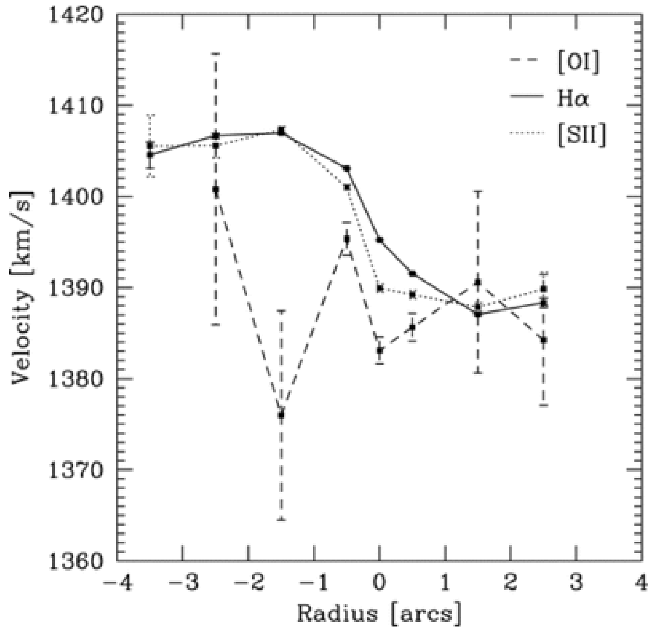
Fig. 6. from An Accreting Black Hole in the Nuclear Star Cluster of the Bulgeless Galaxy NGC 1042 Shields et al. 2008 ApJ 682 104 doi:10.1086/589680 https://dx.doi.org/10.1086/589680
