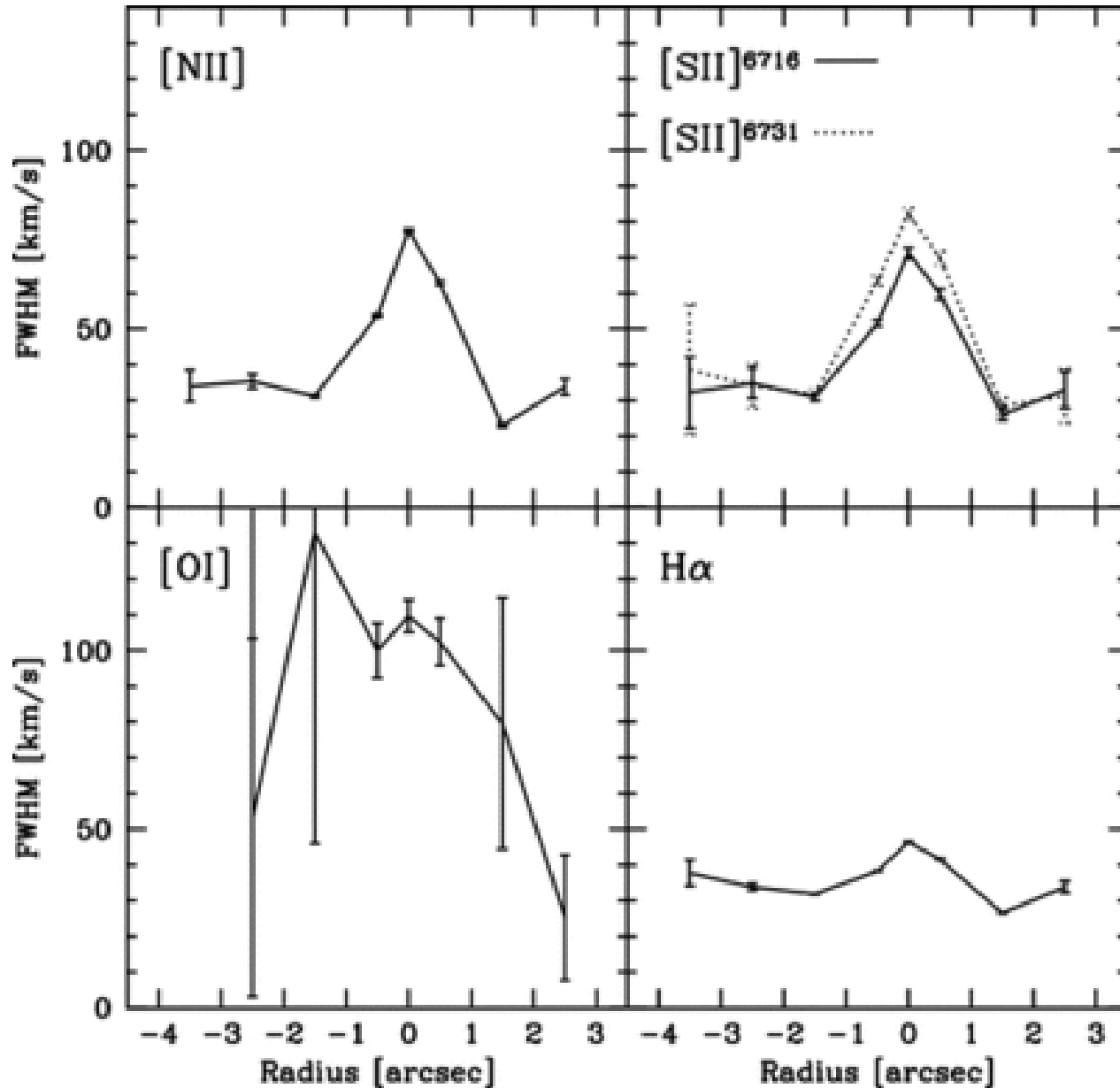
Fig. 5. from An Accreting Black Hole in the Nuclear Star Cluster of the Bulgeless Galaxy NGC 1042 Shields et al. 2008 ApJ 682 104 doi:10.1086/589680 https://dx.doi.org/10.1086/589680
