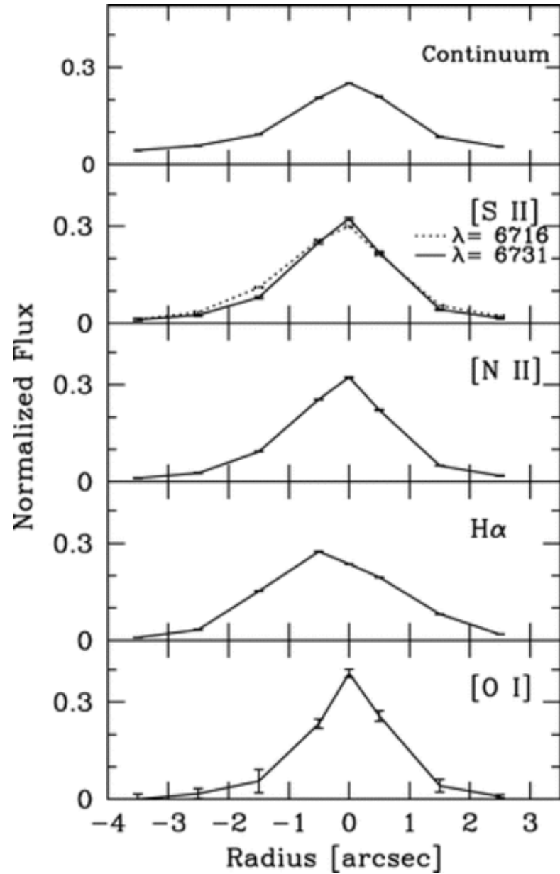
Fig. 4. from An Accreting Black Hole in the Nuclear Star Cluster of the Bulgeless Galaxy NGC 1042 Shields et al. 2008 ApJ 682 104 doi:10.1086/589680 https://dx.doi.org/10.1086/589680
