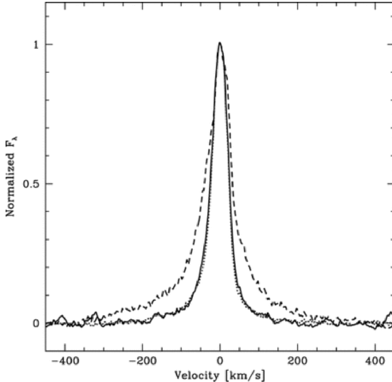
Fig. 3. from An Accreting Black Hole in the Nuclear Star Cluster of the Bulgeless Galaxy NGC 1042 Shields et al. 2008 ApJ 682 104 doi:10.1086/589680 https://dx.doi.org/10.1086/589680 © 2008. The American Astronomical Society. All rights reserved. Printed in U.S.A.
