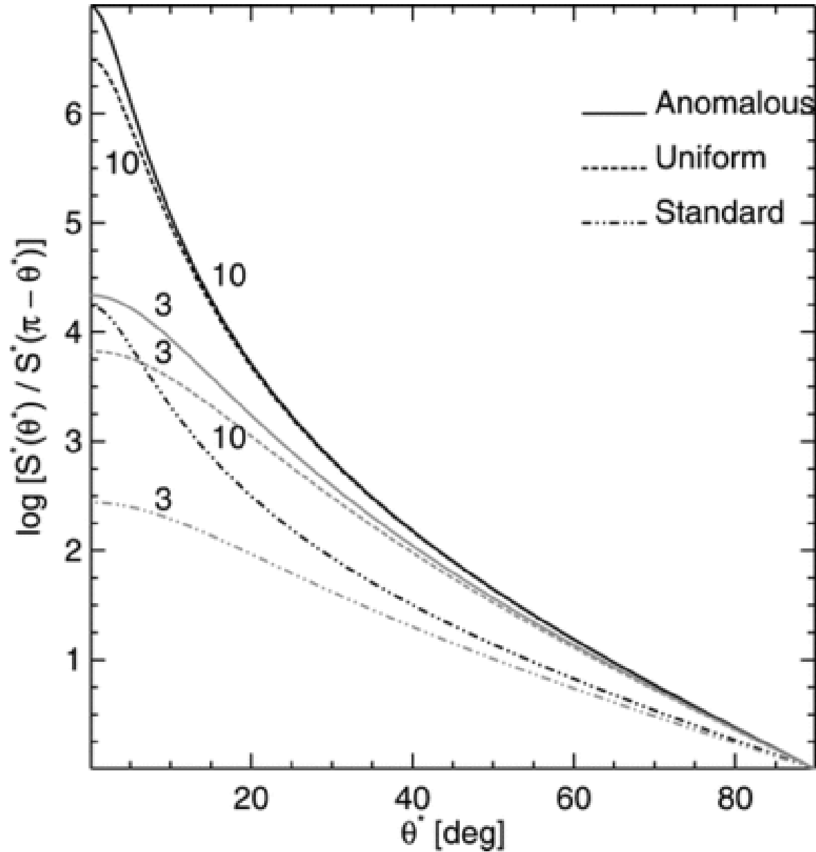
Fig. 8. from Observational Effects of Anomalous Boundary Layers in Relativistic Jets Aloy & Mimica 2008 ApJ 681 84 doi:10.1086/588605 https://dx.doi.org/10.1086/588605 © 2008. The American Astronomical Society. All rights reserved. Printed in U.S.A.
