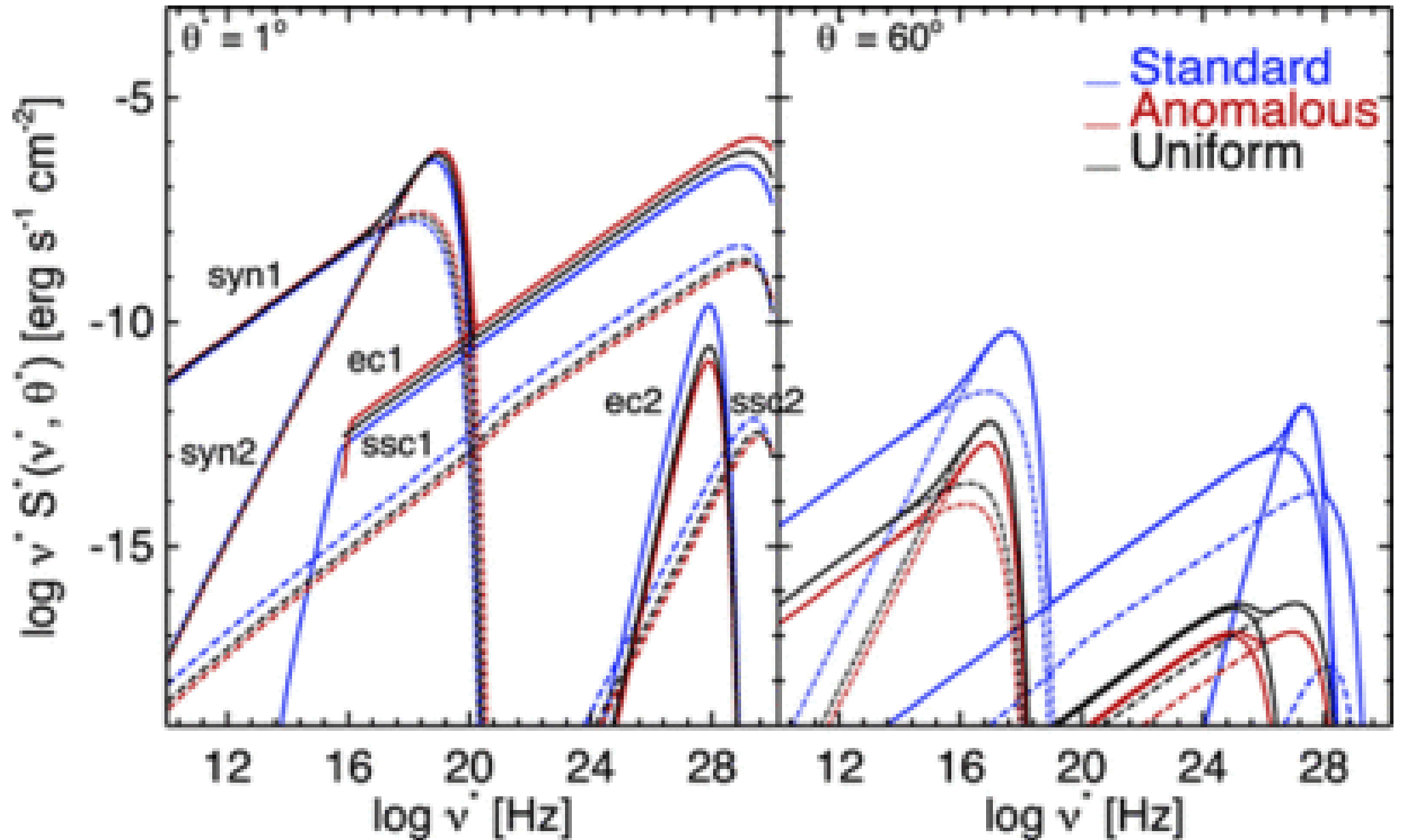
Fig. 5. from Observational Effects of Anomalous Boundary Layers in Relativistic Jets Aloy & Mimica 2008 ApJ 681 84 doi:10.1086/588605 https://dx.doi.org/10.1086/588605 © 2008. The American Astronomical Society. All rights reserved. Printed in U.S.A.
