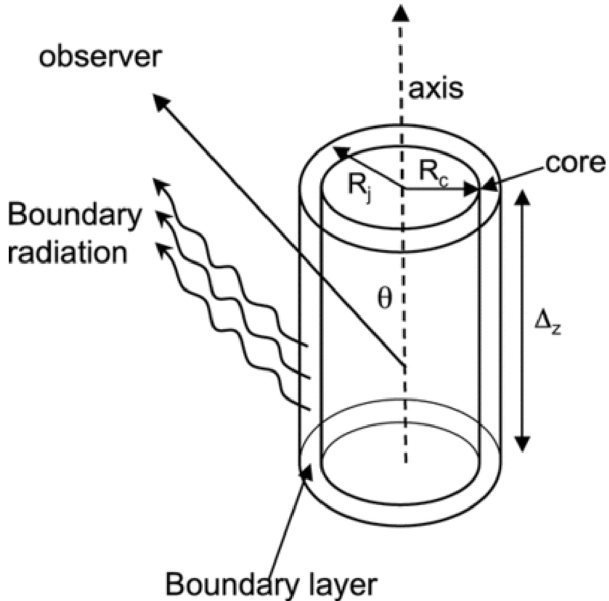
Fig. 4. from Observational Effects of Anomalous Boundary Layers in Relativistic Jets Aloy & Mimica 2008 ApJ 681 84 doi:10.1086/588605 https://dx.doi.org/10.1086/588605 © 2008. The American Astronomical Society. All rights reserved. Printed in U.S.A.
