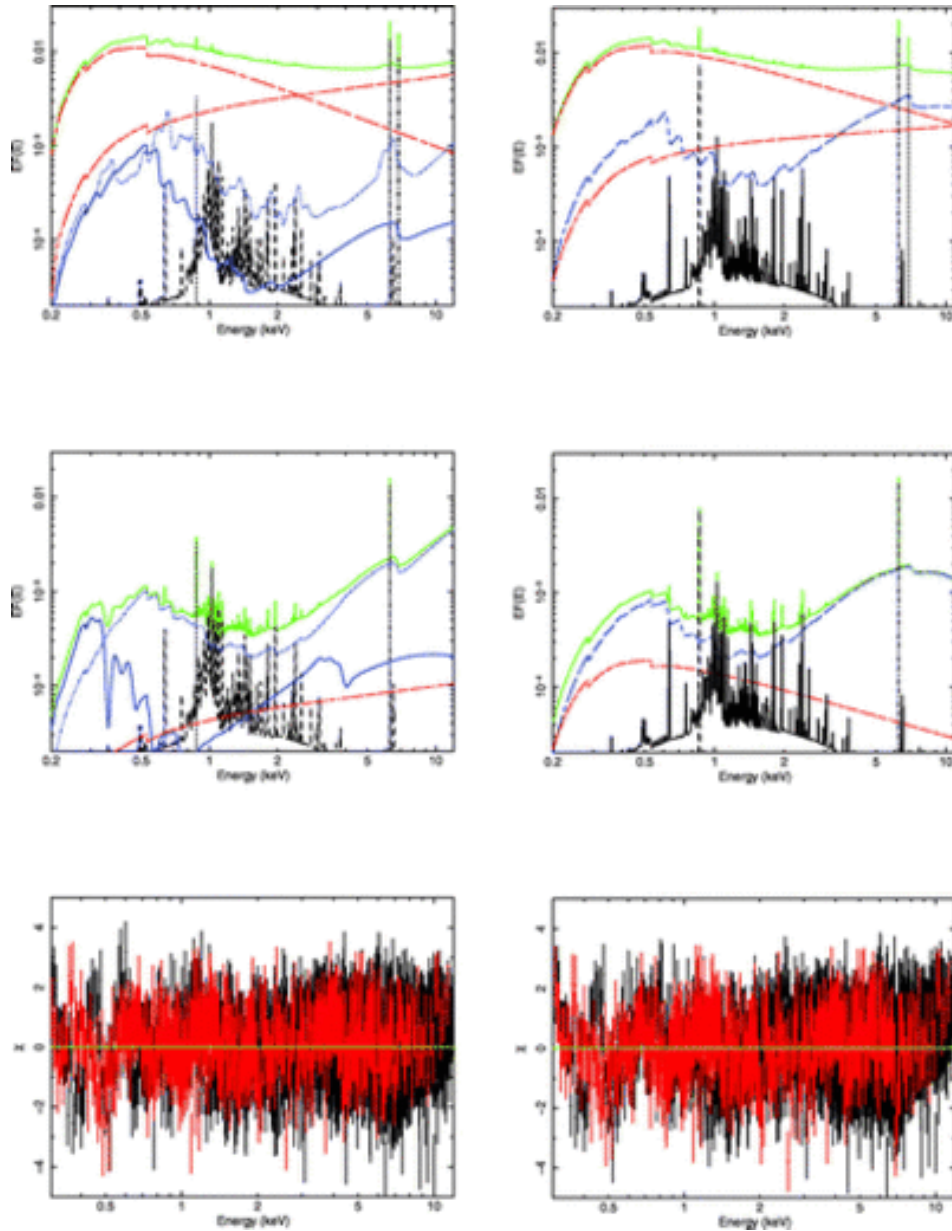
Fig. 7. from XMMNewton Observations of the NarrowLine Seyfert 1 Galaxy Mrk 335 in a Historical Low XRay Flux State Grupe et al. 2008 ApJ 681 982 doi:10.1086/588213 https://dx.doi.org/10.1086/588213
