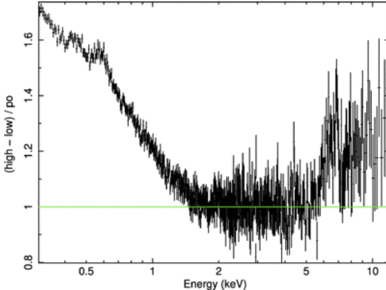
Fig. 6. from XMMNewton Observations of the NarrowLine Seyfert 1 Galaxy Mrk 335 in a Historical Low XRay Flux State Grupe et al. 2008 ApJ 681 982 doi:10.1086/588213 https://dx.doi.org/10.1086/588213 © 2008. The American Astronomical Society. All rights reserved. Printed in U.S.A.
