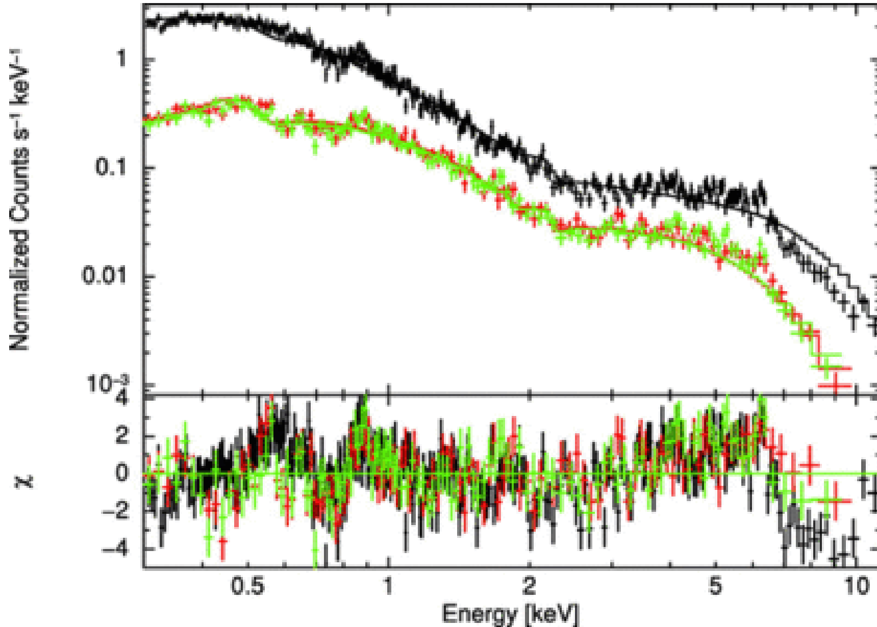
Fig. 4. from XMMNewton Observations of the NarrowLine Seyfert 1 Galaxy Mrk 335 in a Historical Low XRay Flux State Grupe et al. 2008 ApJ 681 982 doi:10.1086/588213 https://dx.doi.org/10.1086/588213 © 2008. The American Astronomical Society. All rights reserved. Printed in U.S.A.
