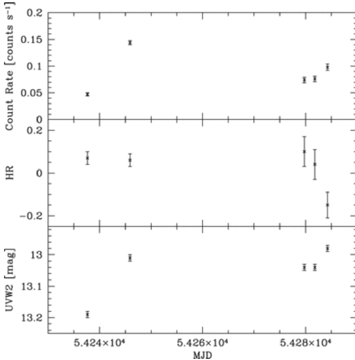
Fig. 3. from XMMNewton Observations of the NarrowLine Seyfert 1 Galaxy Mrk 335 in a Historical Low XRay Flux State Grupe et al. 2008 ApJ 681 982 doi:10.1086/588213 https://dx.doi.org/10.1086/588213
