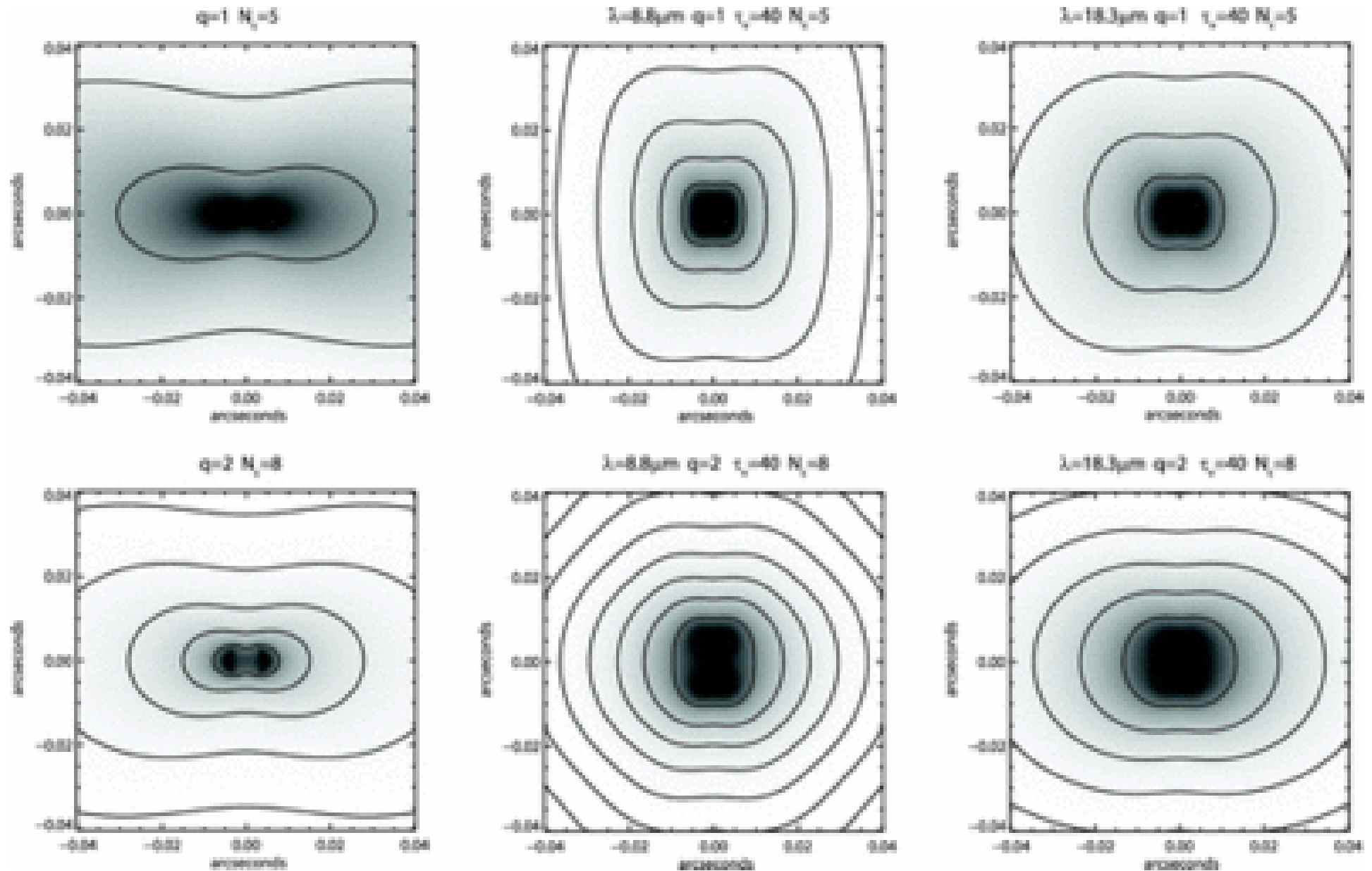
Fig. 6. from Gemini Imaging of MidInfrared Emission from the Nuclear Region of Centaurus A Radomski et al. 2008 ApJ 681 141 doi:10.1086/587771 https://dx.doi.org/10.1086/587771
