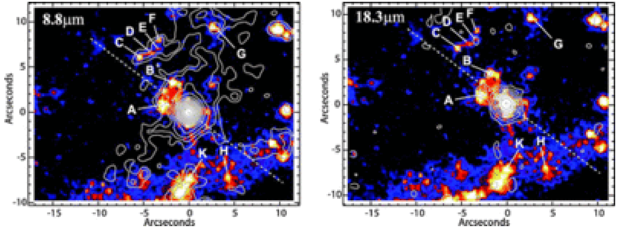
Fig. 3. from Gemini Imaging of MidInfrared Emission from the Nuclear Region of Centaurus A Radomski et al. 2008 ApJ 681 141 doi:10.1086/587771 https://dx.doi.org/10.1086/587771 © 2008. The American Astronomical Society. All rights reserved. Printed in U.S.A.
