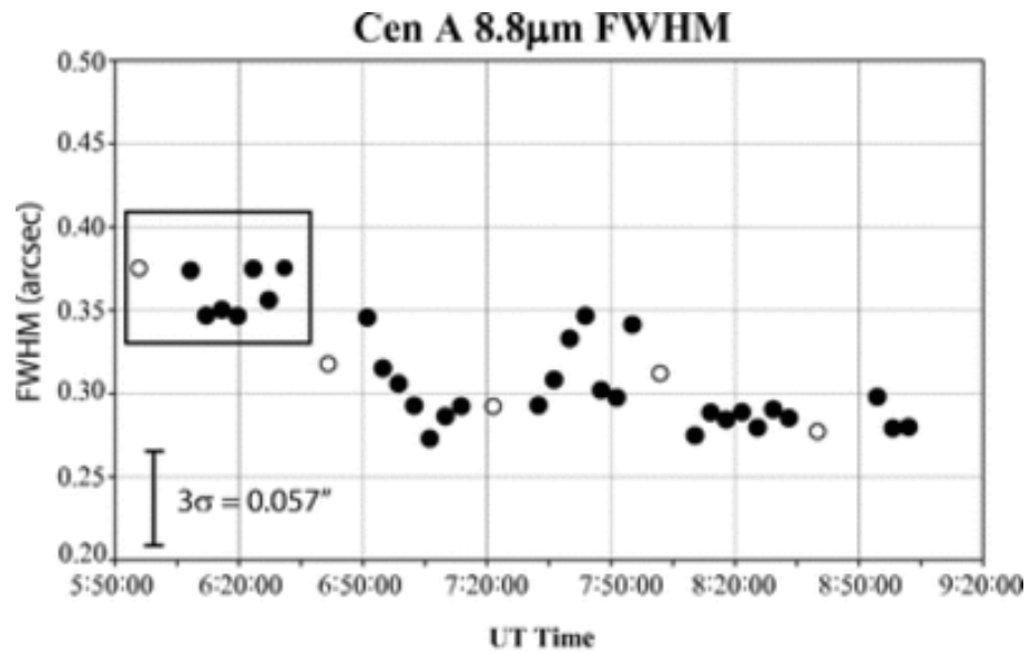
Fig. 1. from Gemini Imaging of MidInfrared Emission from the Nuclear Region of Centaurus A Radomski et al. 2008 ApJ 681 141 doi:10.1086/587771 https://dx.doi.org/10.1086/587771
