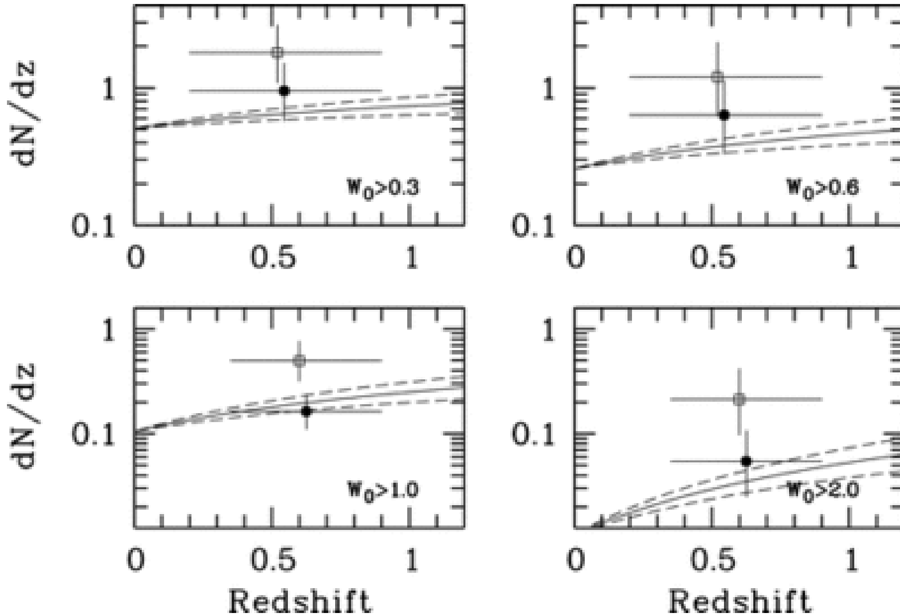
Fig. 5. from Galaxy Clusters in the Line of Sight to Background Quasars. I. Survey Design and Incidence of Mg II Absorbers at Cluster Redshifts Lopez et al. 2008 ApJ 679 1144 doi:10.1086/587678 https://dx.doi.org/10.1086/587678 © 2008. The American Astronomical Society. All rights reserved. Printed in U.S.A.
