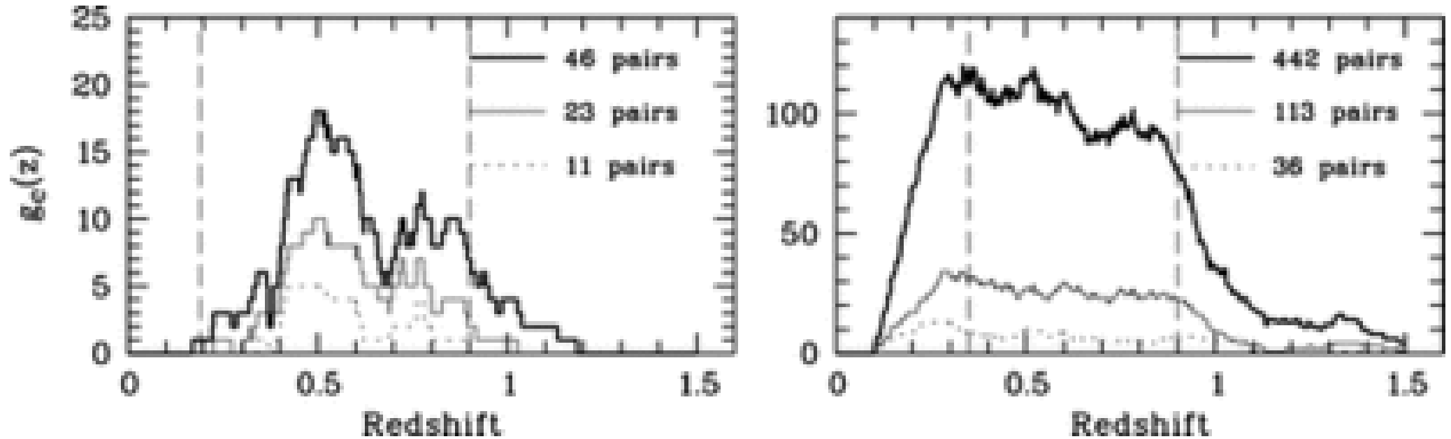
Fig. 4. from Galaxy Clusters in the Line of Sight to Background Quasars. I. Survey Design and Incidence of Mg II Absorbers at Cluster Redshifts Lopez et al. 2008 ApJ 679 1144 doi:10.1086/587678 https://dx.doi.org/10.1086/587678
