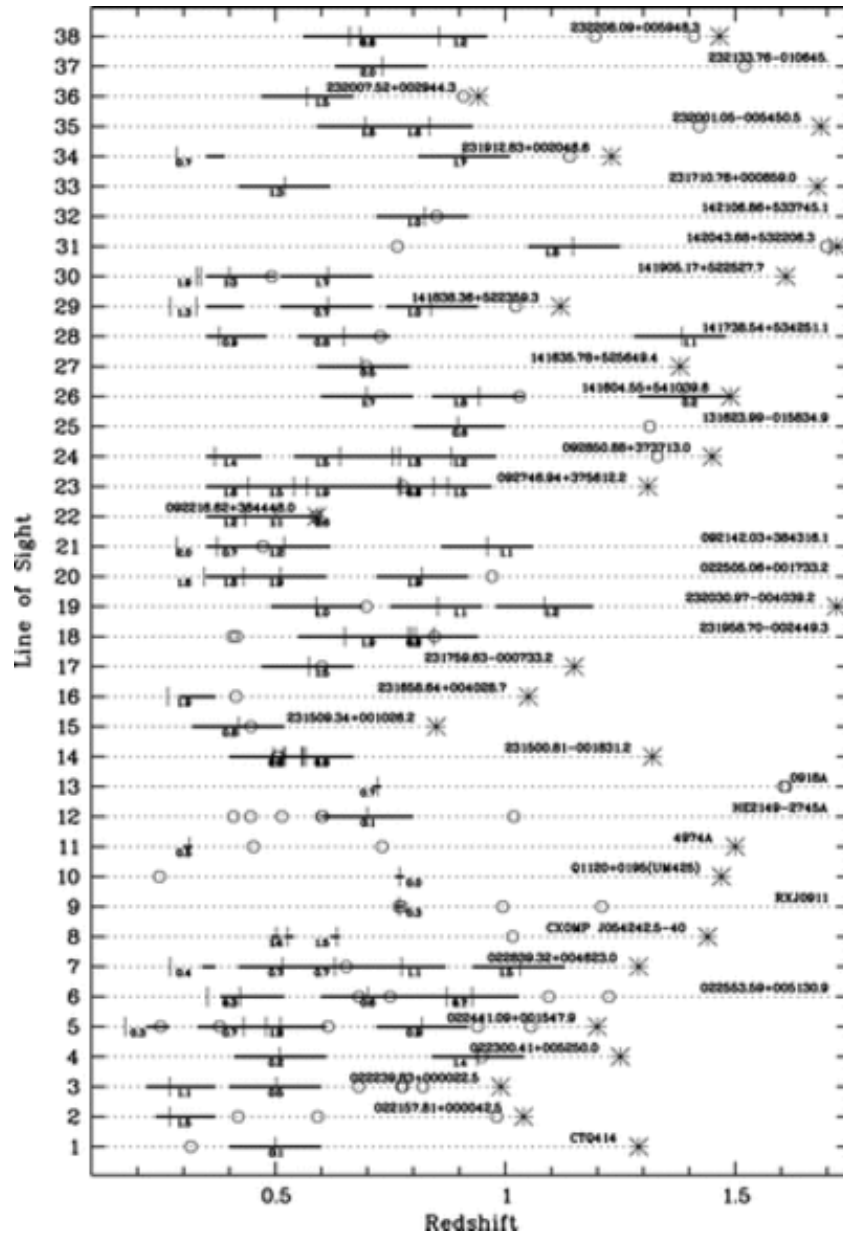
Fig. 3. from Galaxy Clusters in the Line of Sight to Background Quasars. I. Survey Design and Incidence of Mg II Absorbers at Cluster Redshifts Lopez et al. 2008 ApJ 679 1144 doi:10.1086/587678 https://dx.doi.org/10.1086/587678 © 2008. The American Astronomical Society. All rights reserved. Printed in U.S.A.
