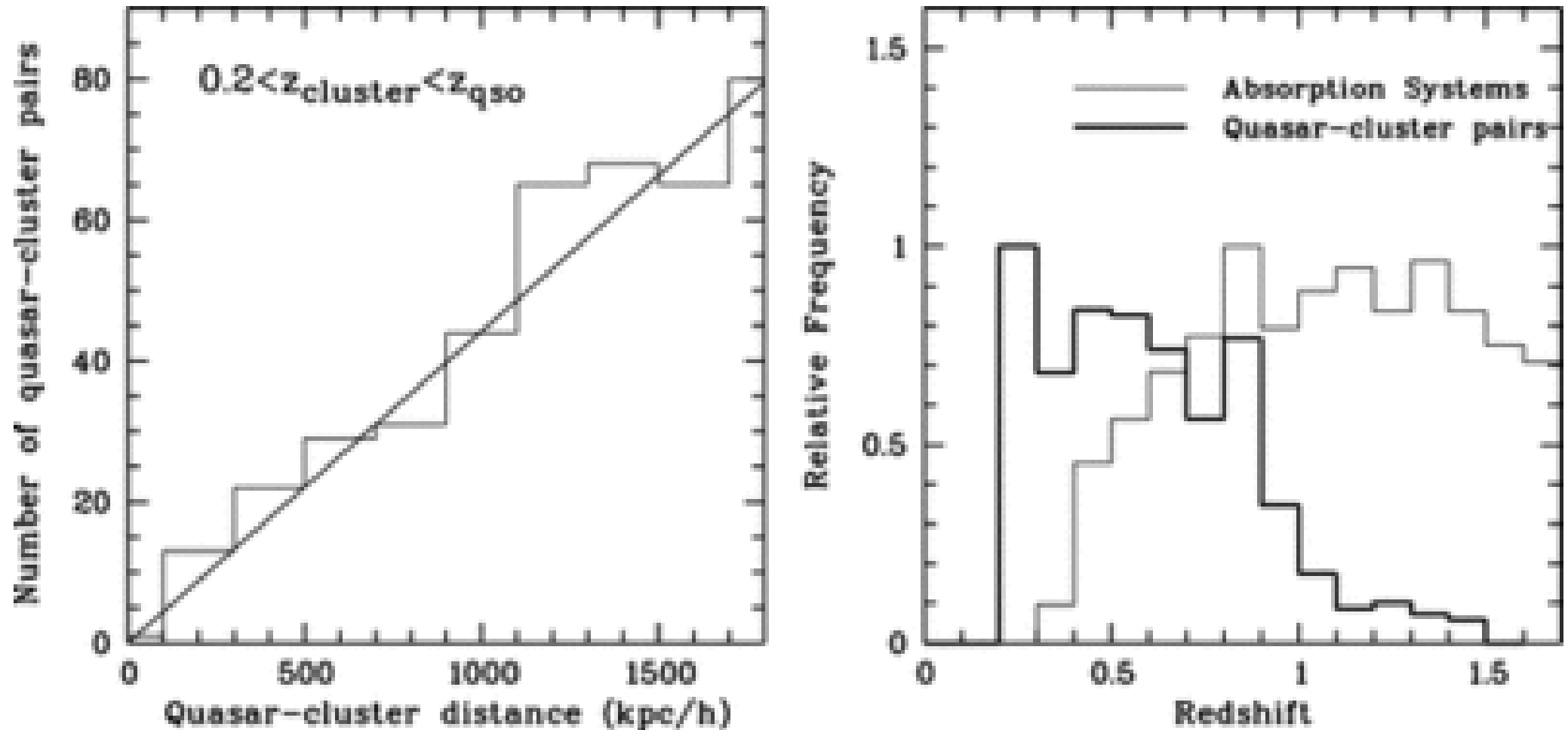
Fig. 1. from Galaxy Clusters in the Line of Sight to Background Quasars. I. Survey Design and Incidence of Mg II Absorbers at Cluster Redshifts Lopez et al. 2008 ApJ 679 1144 doi:10.1086/587678 https://dx.doi.org/10.1086/587678 © 2008. The American Astronomical Society. All rights reserved. Printed in U.S.A.
