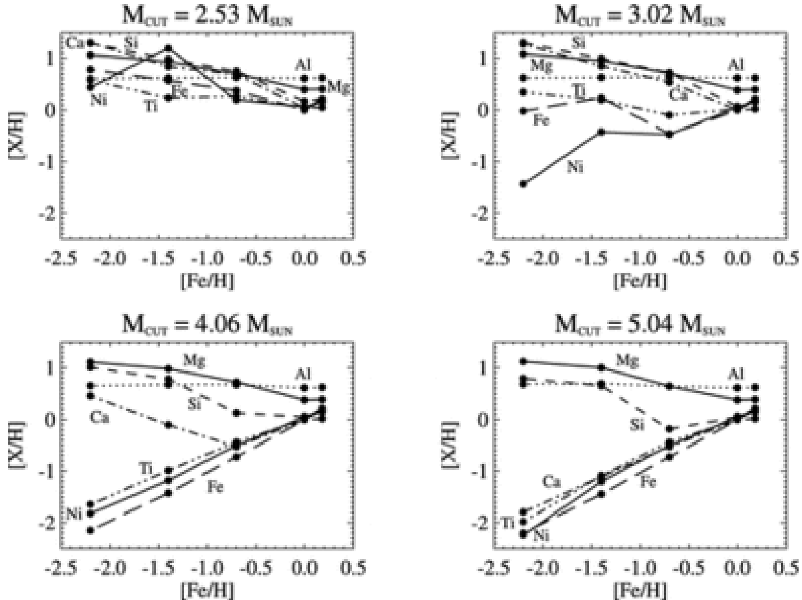
Fig. 8. from Chemical Abundances of the Secondary Star in the Black Hole XRay Binary XTE J1118+480 González Hernández et al. 2008 ApJ 679 732 doi:10.1086/586888 https://dx.doi.org/10.1086/586888 © 2008. The American Astronomical Society. All rights reserved. Printed in U.S.A.
