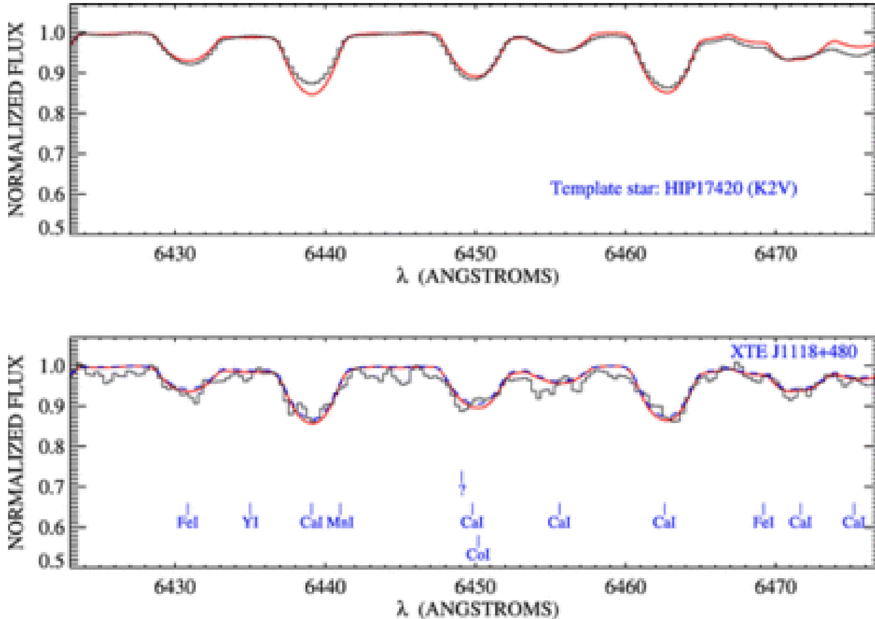
Fig. 6. from Chemical Abundances of the Secondary Star in the Black Hole XRay Binary XTE J1118+480 González Hernández et al. 2008 ApJ 679 732 doi:10.1086/586888 https://dx.doi.org/10.1086/586888 © 2008. The American Astronomical Society. All rights reserved. Printed in U.S.A.
