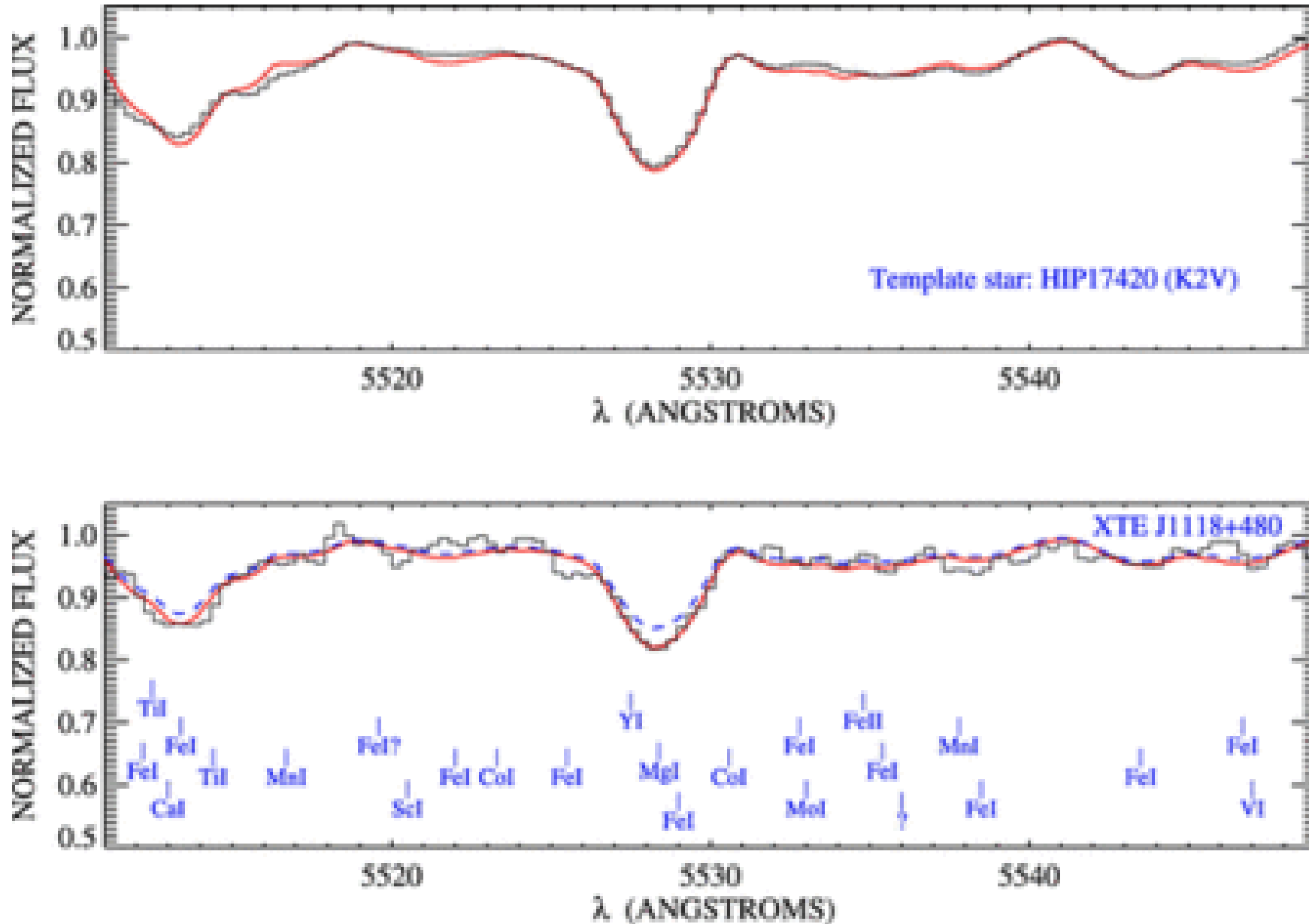
Fig. 5. from Chemical Abundances of the Secondary Star in the Black Hole XRay Binary XTE J1118+480 González Hernández et al. 2008 ApJ 679 732 doi:10.1086/586888 https://dx.doi.org/10.1086/586888 © 2008. The American Astronomical Society. All rights reserved. Printed in U.S.A.
