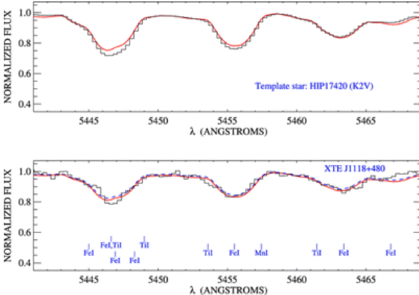
Fig. 4. from Chemical Abundances of the Secondary Star in the Black Hole XRay Binary XTE J1118+480 González Hernández et al. 2008 ApJ 679 732 doi:10.1086/586888 https://dx.doi.org/10.1086/586888 © 2008. The American Astronomical Society. All rights reserved. Printed in U.S.A.
