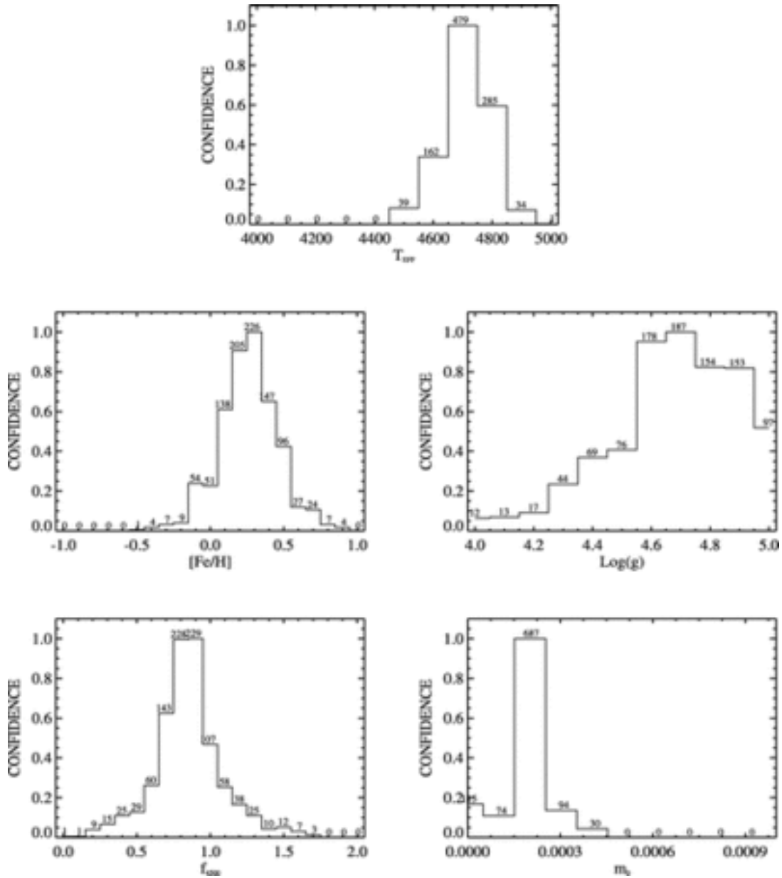
Fig. 3. from Chemical Abundances of the Secondary Star in the Black Hole XRay Binary XTE J1118+480 González Hernández et al. 2008 ApJ 679 732 doi:10.1086/586888 https://dx.doi.org/10.1086/586888 © 2008. The American Astronomical Society. All rights reserved. Printed in U.S.A.
