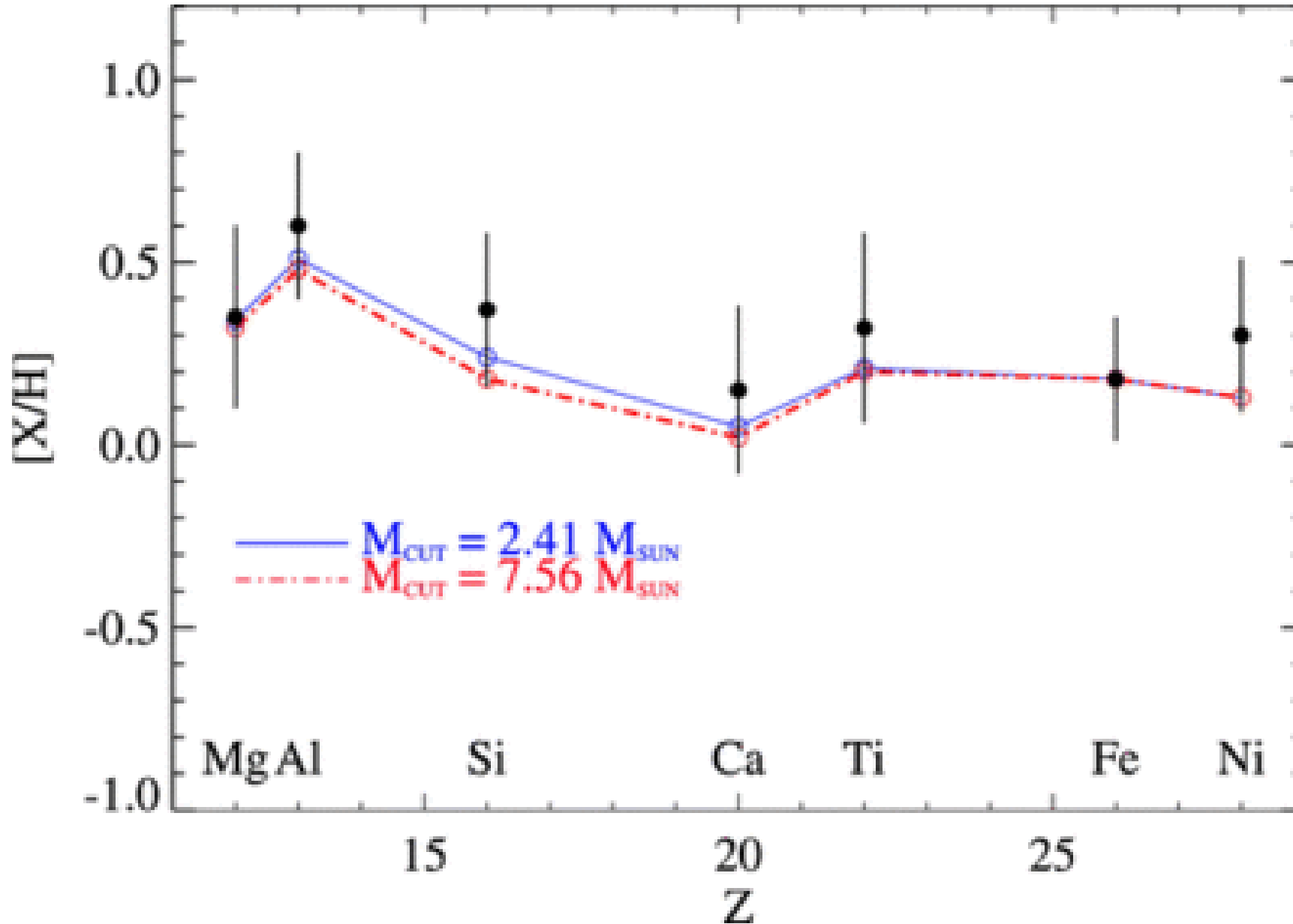
Fig. 13. from Chemical Abundances of the Secondary Star in the Black Hole XRay Binary XTE J1118+480 González Hernández et al. 2008 ApJ 679 732 doi:10.1086/586888 https://dx.doi.org/10.1086/586888 © 2008. The American Astronomical Society. All rights reserved. Printed in U.S.A.
