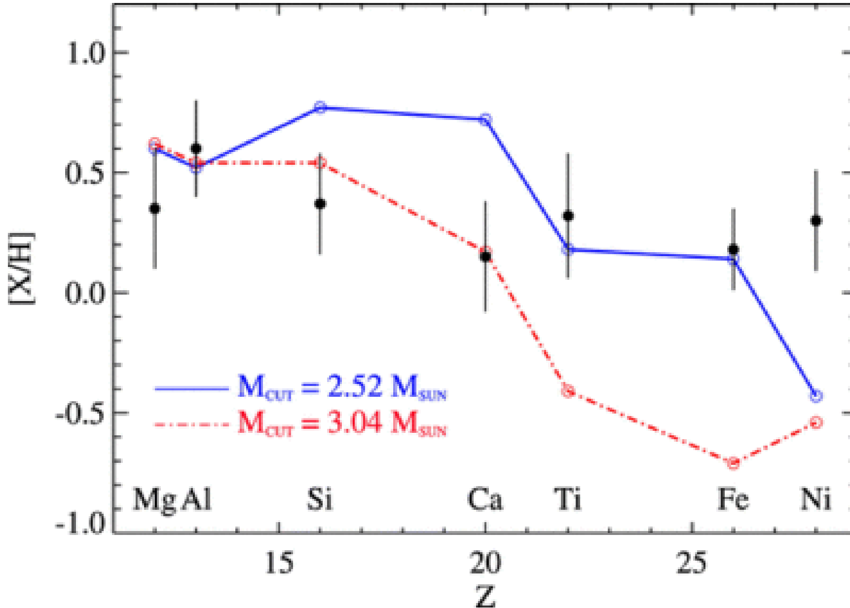
Fig. 11. from Chemical Abundances of the Secondary Star in the Black Hole XRay Binary XTE J1118+480 González Hernández et al. 2008 ApJ 679 732 doi:10.1086/586888 https://dx.doi.org/10.1086/586888 © 2008. The American Astronomical Society. All rights reserved. Printed in U.S.A.
