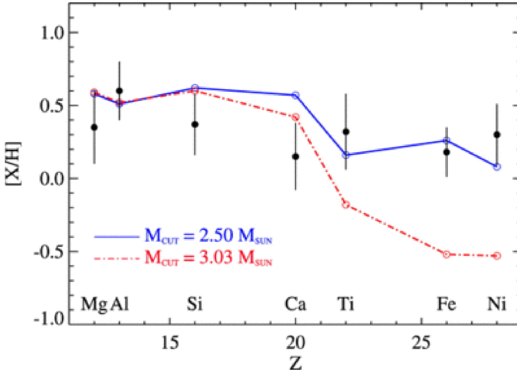
Fig. 10. from Chemical Abundances of the Secondary Star in the Black Hole XRay Binary XTE J1118+480 González Hernández et al. 2008 ApJ 679 732 doi:10.1086/586888 https://dx.doi.org/10.1086/586888 © 2008. The American Astronomical Society. All rights reserved. Printed in U.S.A.
