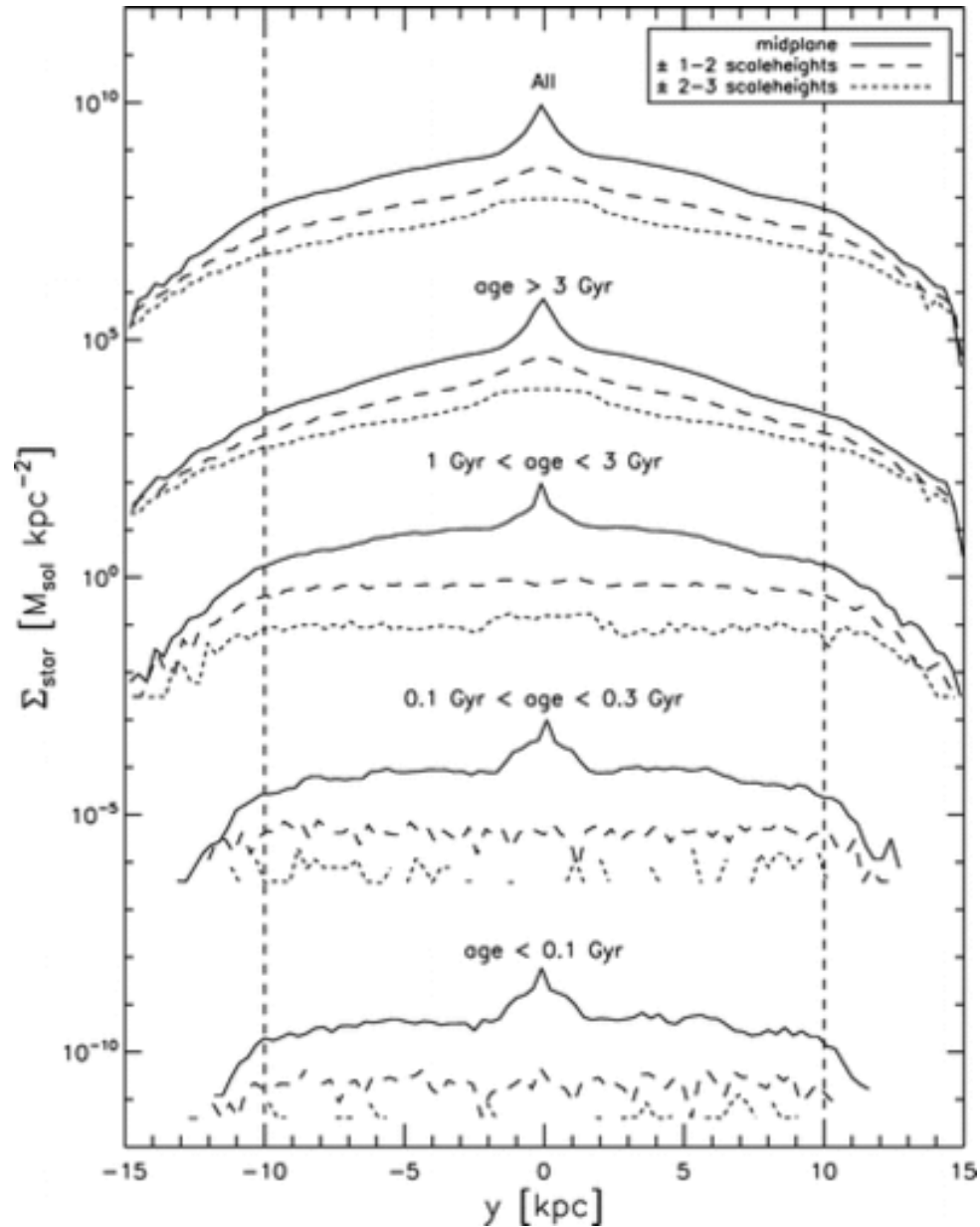
Fig. 3. from Beyond InsideOut Growth: Formation and Evolution of Disk Outskirts Roškar et al. 2008 ApJL 675 L65 doi:10.1086/586734 https://dx.doi.org/10.1086/586734 © 2008. The American Astronomical Society. All rights reserved. Printed in U.S.A.
