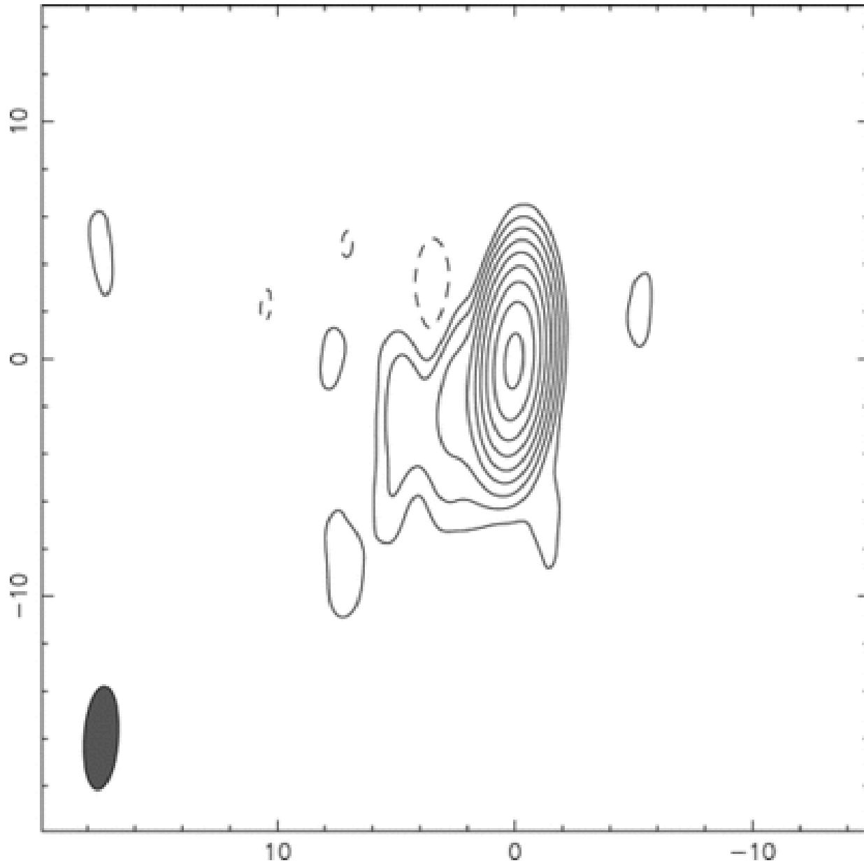
Fig. 9. from The ParsecScale Jets of the TeV Blazars H1426+428, 1ES 1959+650, and PKS 2155304: 2001–2004 Piner, Pant, & Edwards 2008 ApJ 678 64 doi:10.1086/533521 https://dx.doi.org/10.1086/533521 © 2008. The American Astronomical Society. All rights reserved. Printed in U.S.A.
