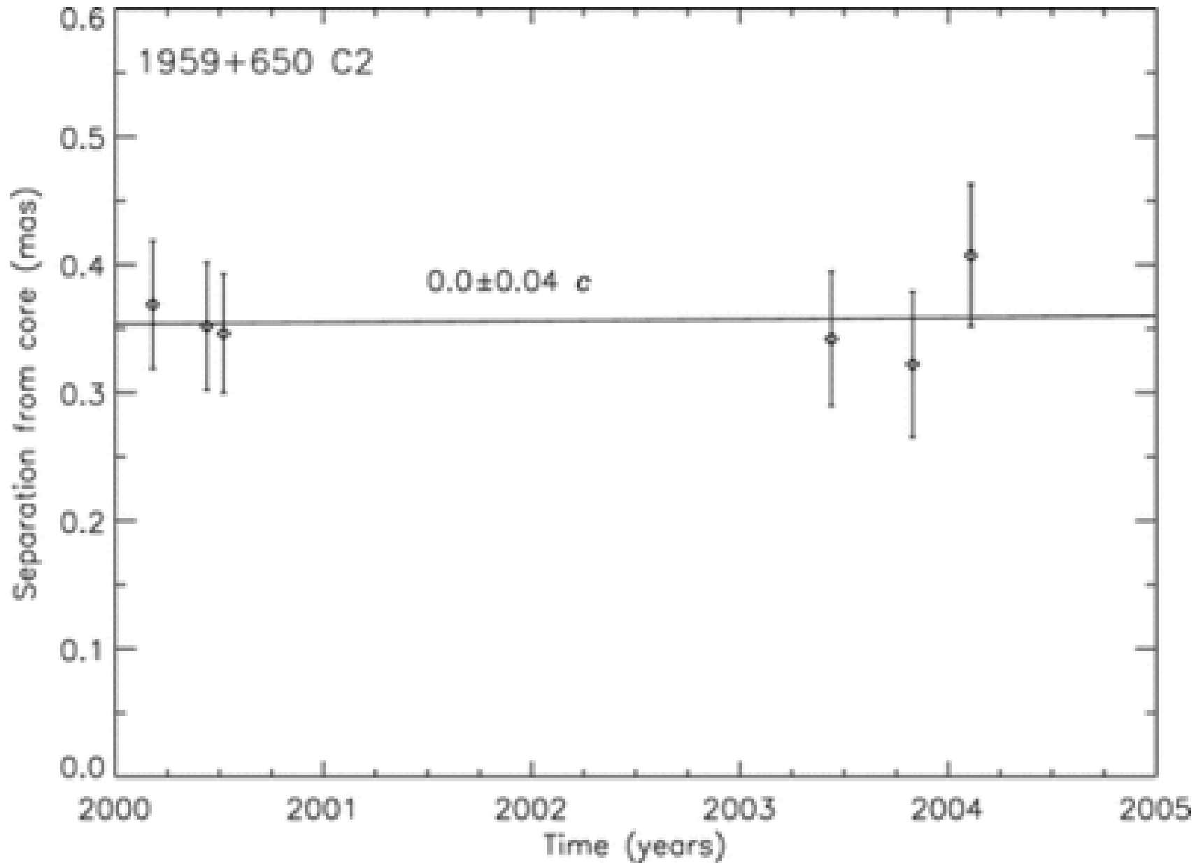
Fig. 7. from The ParsecScale Jets of the TeV Blazars H1426+428, 1ES 1959+650, and PKS 2155304: 2001–2004 Piner, Pant, & Edwards 2008 ApJ 678 64 doi:10.1086/533521 https://dx.doi.org/10.1086/533521
