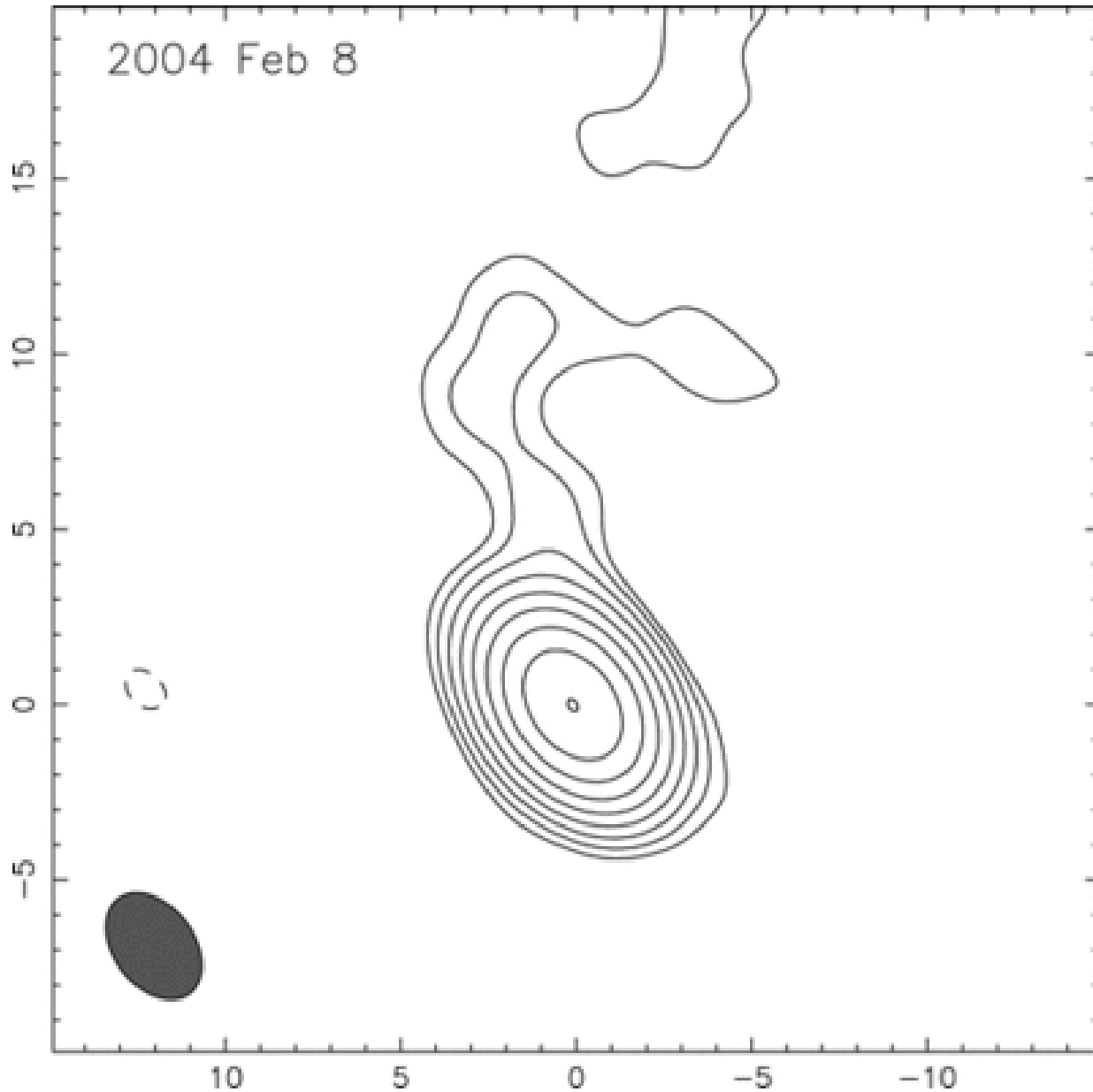
Fig. 5. from The ParsecScale Jets of the TeV Blazars H1426+428, 1ES 1959+650, and PKS 2155304: 2001–2004 Piner, Pant, & Edwards 2008 ApJ 678 64 doi:10.1086/533521 https://dx.doi.org/10.1086/533521 © 2008. The American Astronomical Society. All rights reserved. Printed in U.S.A.
