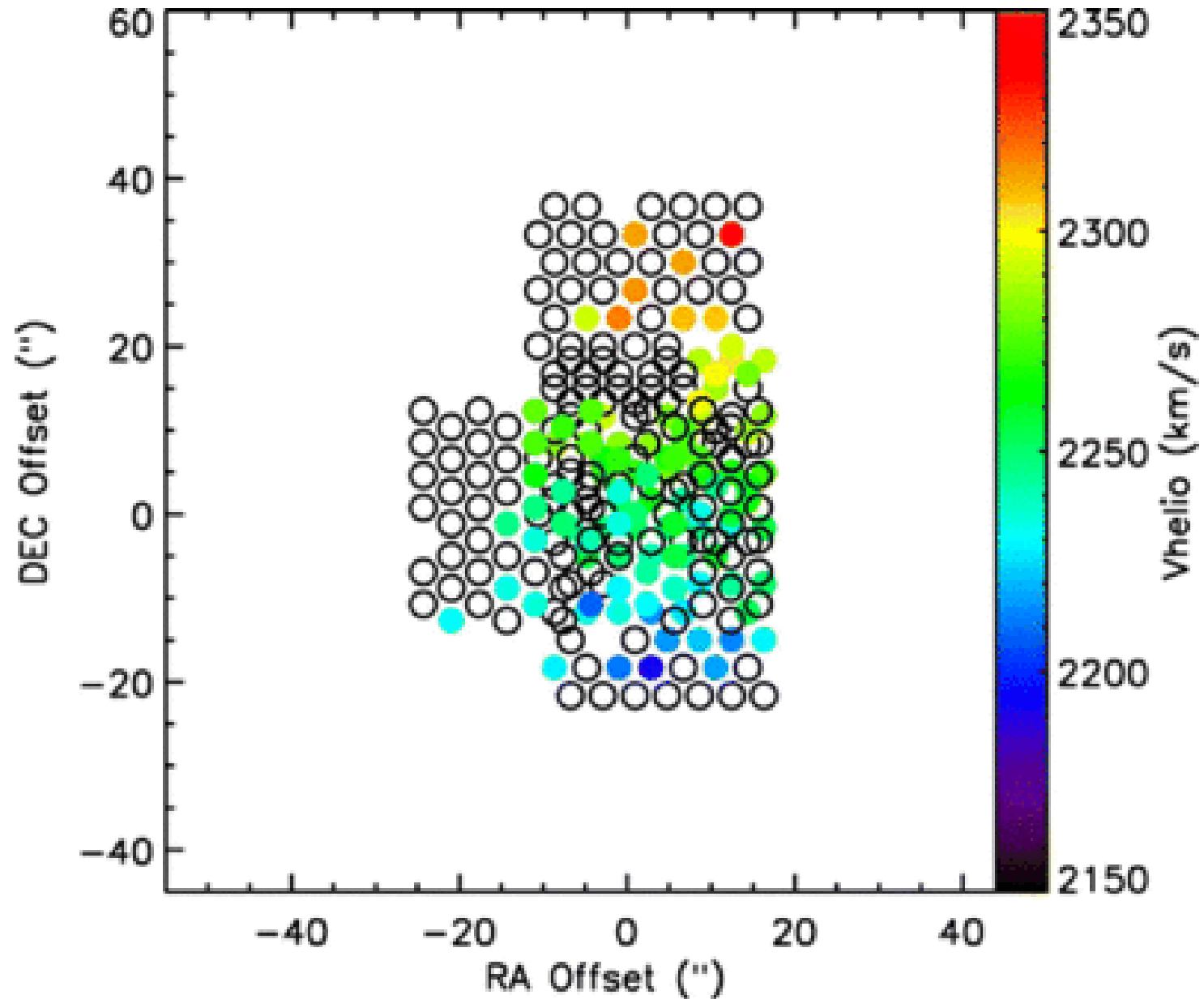
Fig. 1. from Mass Models for Low Surface Brightness Galaxies with HighResolution Optical Velocity Fields Kuzio de Naray, McGaugh, & de Blok 2008 ApJ 676 920 doi:10.1086/527543 https://dx.doi.org/10.1086/527543
