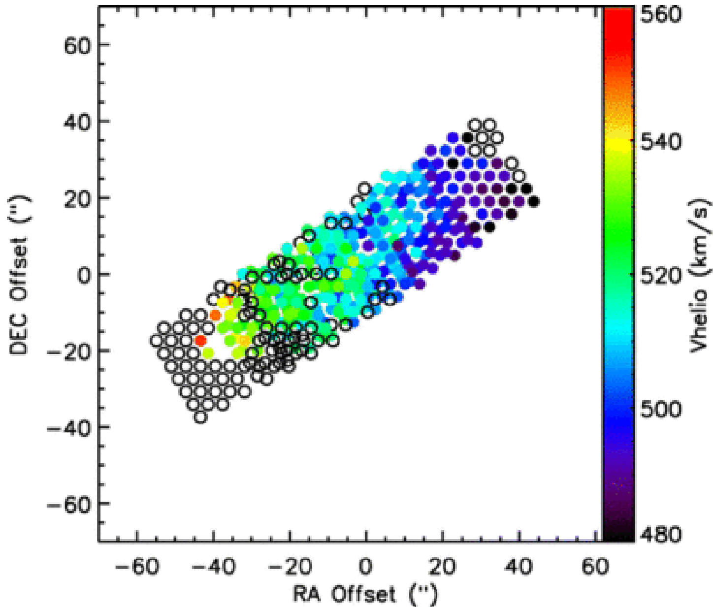
Fig. 1. from Mass Models for Low Surface Brightness Galaxies with HighResolution Optical Velocity Fields Kuzio de Naray, McGaugh, & de Blok 2008 ApJ 676 920 doi:10.1086/527543 https://dx.doi.org/10.1086/527543 © 2008. The American Astronomical Society. All rights reserved. Printed in U.S.A.
