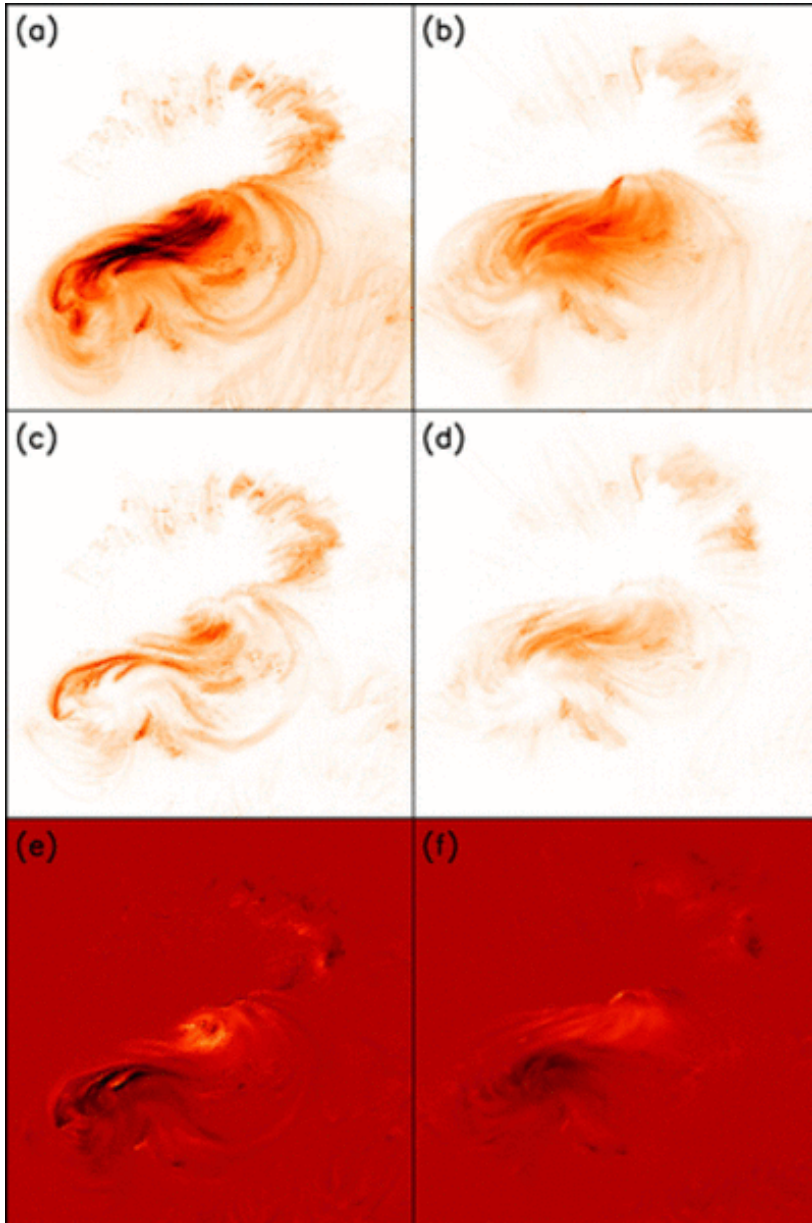
Fig. 4. from Nonlinear Forcefree Field Modeling of a Solar Active Region around the Time of a Major Flare and Coronal Mass Ejection Schrijver et al. 2008 ApJ 675 1637 doi:10.1086/527413 https://dx.doi.org/10.1086/527413
