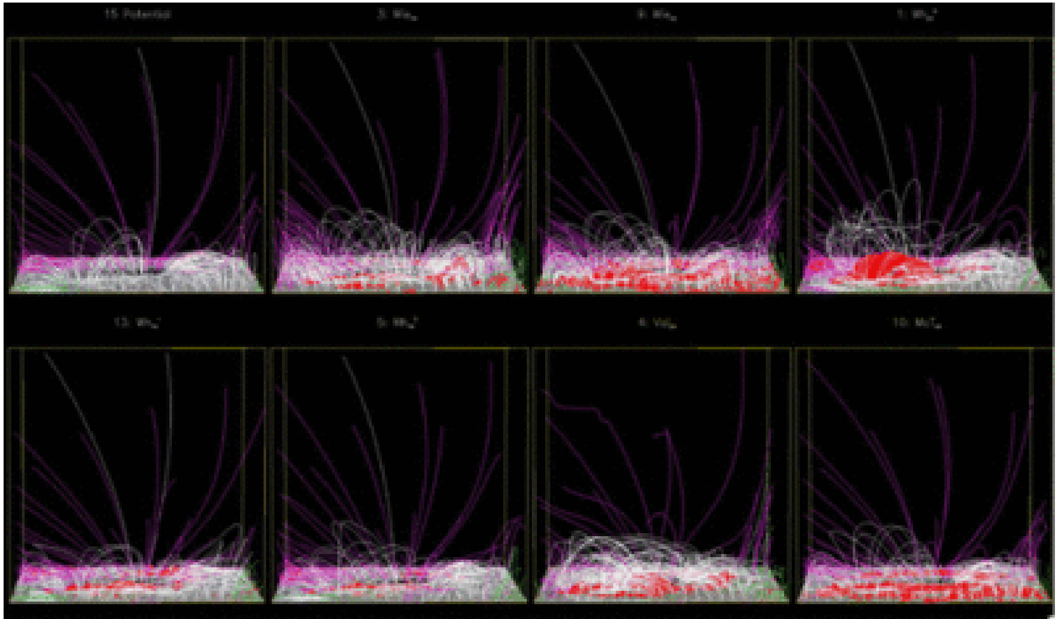
Fig. 3. from Nonlinear Forcefree Field Modeling of a Solar Active Region around the Time of a Major Flare and Coronal Mass Ejection Schrijver et al. 2008 ApJ 675 1637 doi:10.1086/527413 https://dx.doi.org/10.1086/527413 © 2008. The American Astronomical Society. All rights reserved. Printed in U.S.A.
