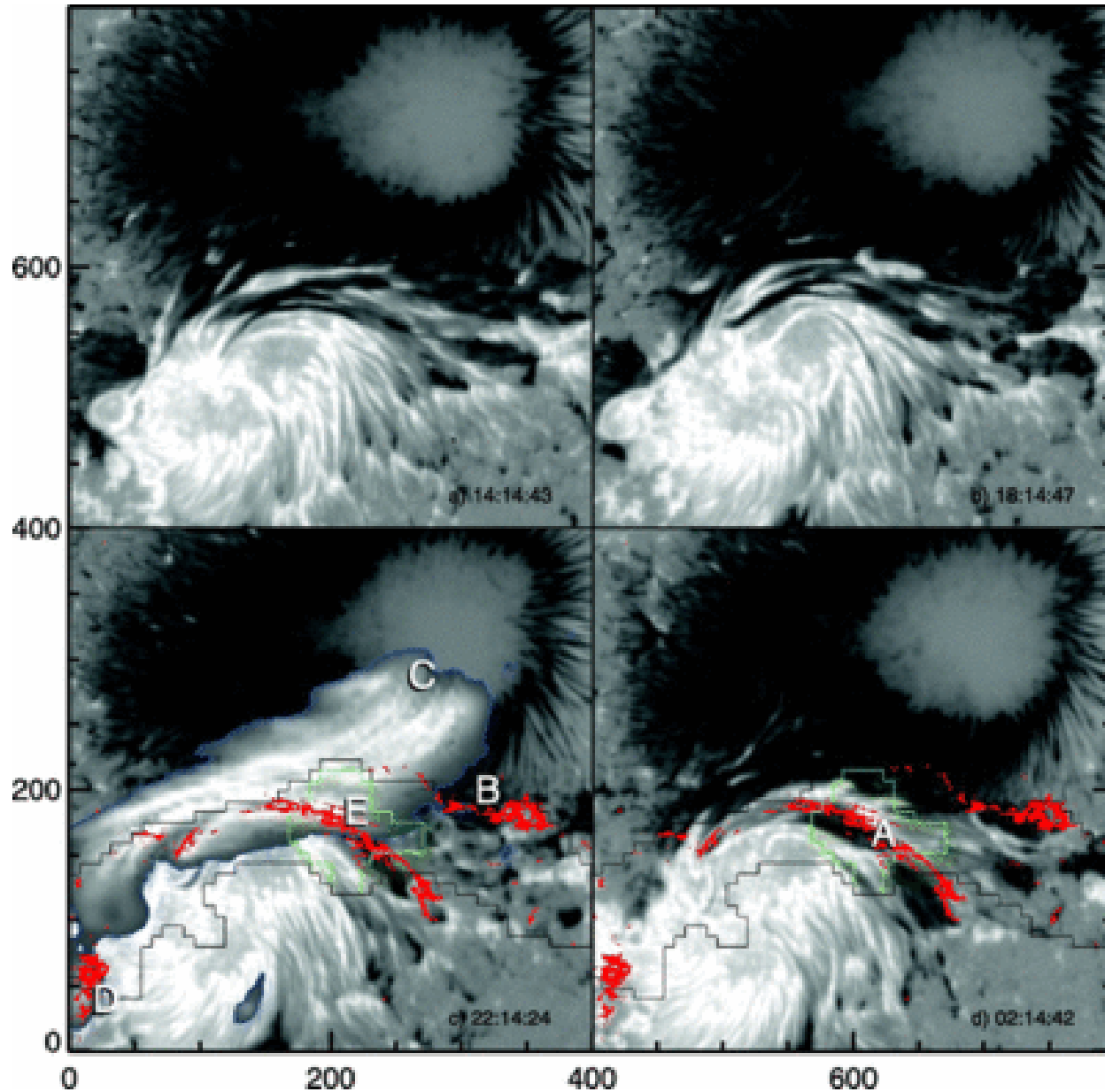
Fig. 2. from Nonlinear Forcefree Field Modeling of a Solar Active Region around the Time of a Major Flare and Coronal Mass Ejection Schrijver et al. 2008 ApJ 675 1637 doi:10.1086/527413 https://dx.doi.org/10.1086/527413 © 2008. The American Astronomical Society. All rights reserved. Printed in U.S.A.
